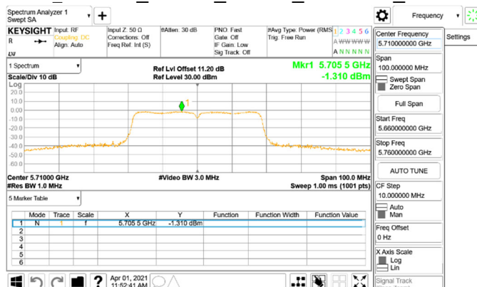
PSD_802.11n_40MHz_Chain0_5710MHz_UNII 2C
