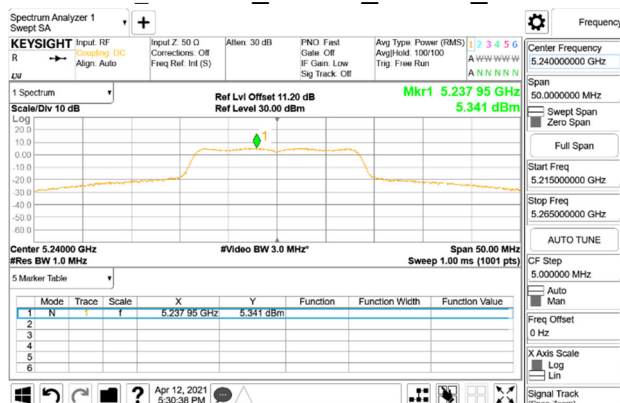
PSD_802.11a_20MHz_Chain0_5240MHz
