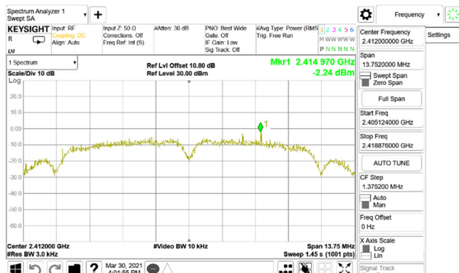
Power Density_802.11b_20MHz_Chain0_2412MHz
