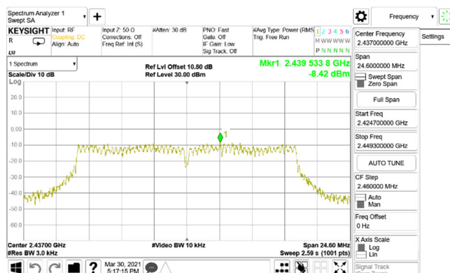
Power Density_802.11g_20MHz_Chain0_2437MHz
