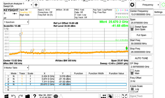
Spurious Emission_802.11g_20MHz_Chain0_2437MHz
