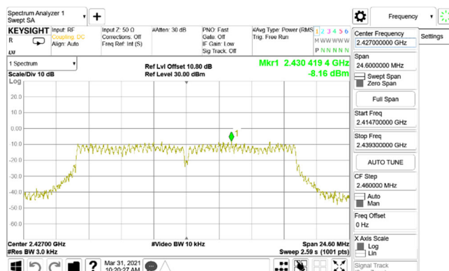
Power Density_802.11g_20MHz_Chain0_2427MHz
