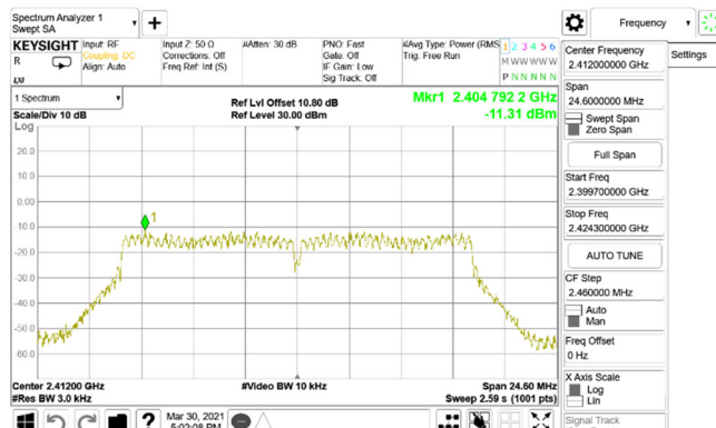
Power Density_802.11g_20MHz_Chain0_2412MHz
