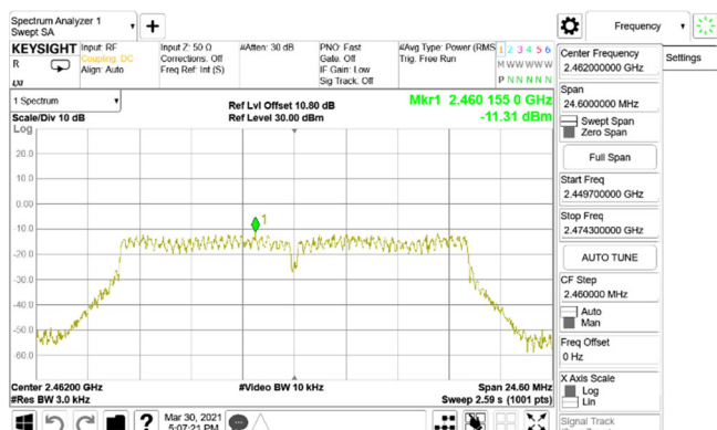
Power Density_802.11g_20MHz_Chain0_2462MHz
