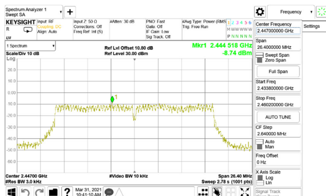
Power Density_802.11n_20MHz_Chain0_2447MHz
