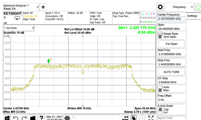
Power Density_802.11n_20MHz_Chain0_2427MHz
