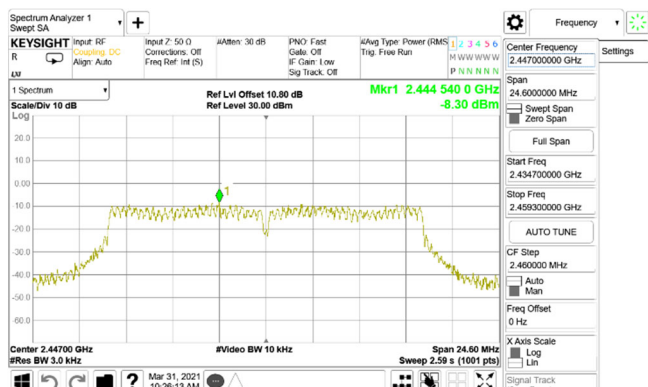
Power Density_802.11g_20MHz_Chain0_2447MHz
