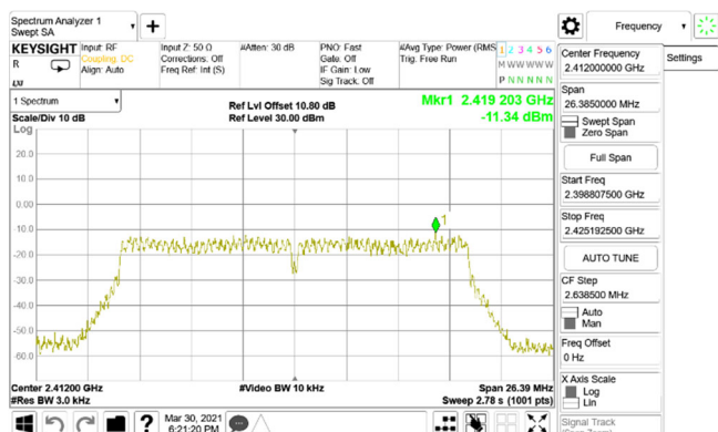
Power Density_802.11n_20MHz_Chain0_2412MHz
