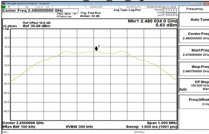
Reference Level BLE 1M HighCH39-2480
