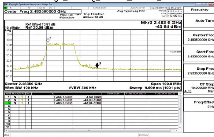
Band Edge_802.11g_20MHz_Chain0_2462MHz
