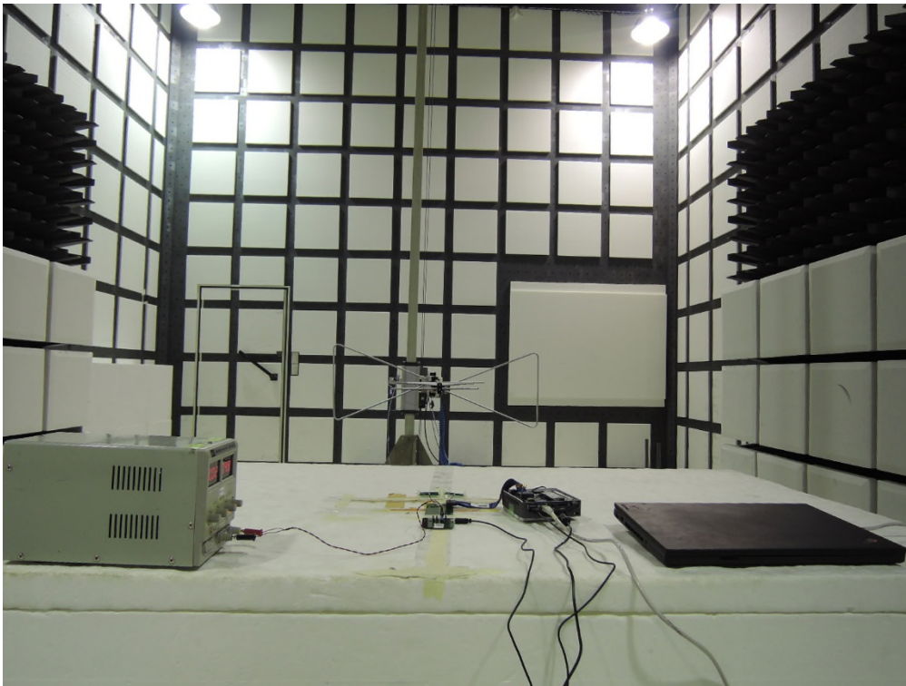
Radiated Emission Set up Photos (Below 1GHz)
