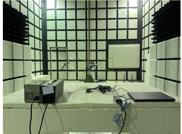
Part_15_247_WLAN_2.4G_Radiated_Setup
