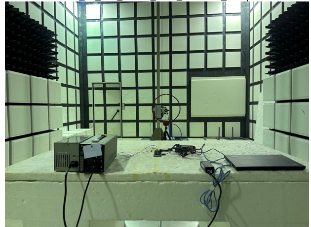
Part_15_247_WLAN_2.4G_Radiated_Setup
