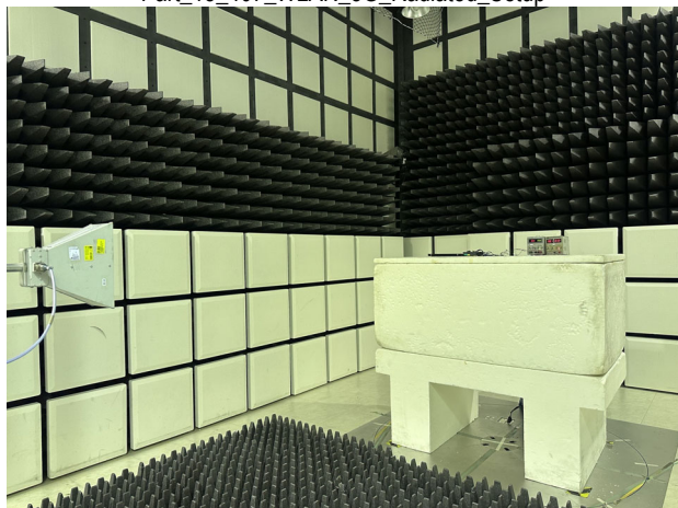
Part_15_407_WLAN_5G_Radiated_Setup
