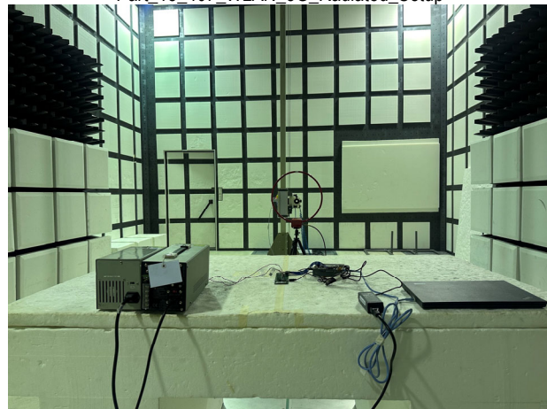
Part_15_407_WLAN_5G_Conducted_Setup
