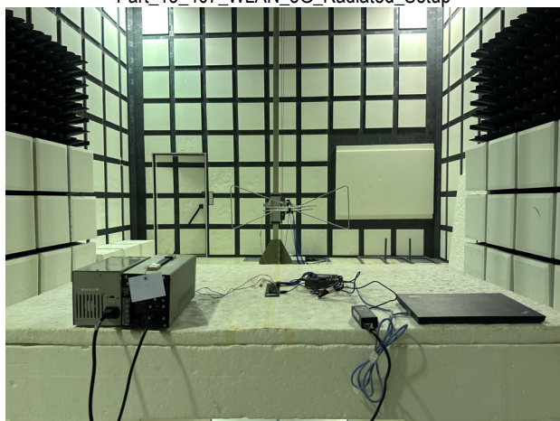
Part_15_407_WLAN_5G_Radiated_Setup
