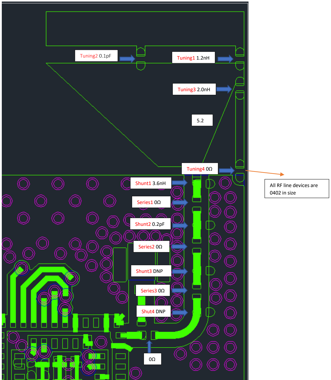
RF matching
