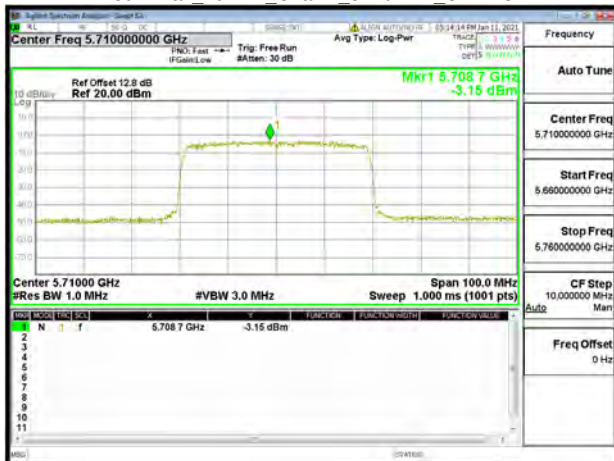
802.11ax_40MHz_Chain1_5710MHz_UNII 2C
