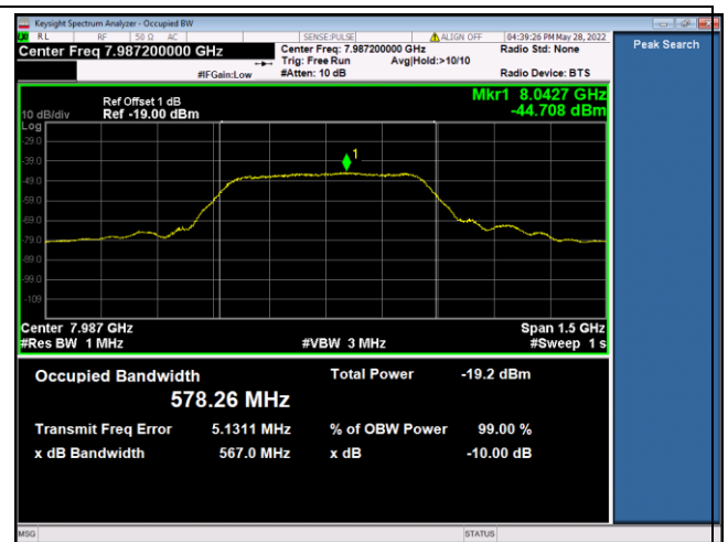
7987.2MHz_HPRF2_SP 1_STS 1_Payload 2
