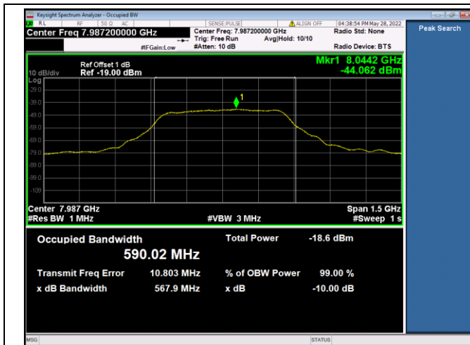
7987.2MHz_HPRF2_SP 0_Payload 1023
