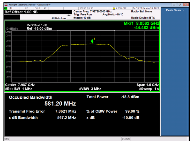
7987.2MHz_HPRF1_SP 0_Payload 512
