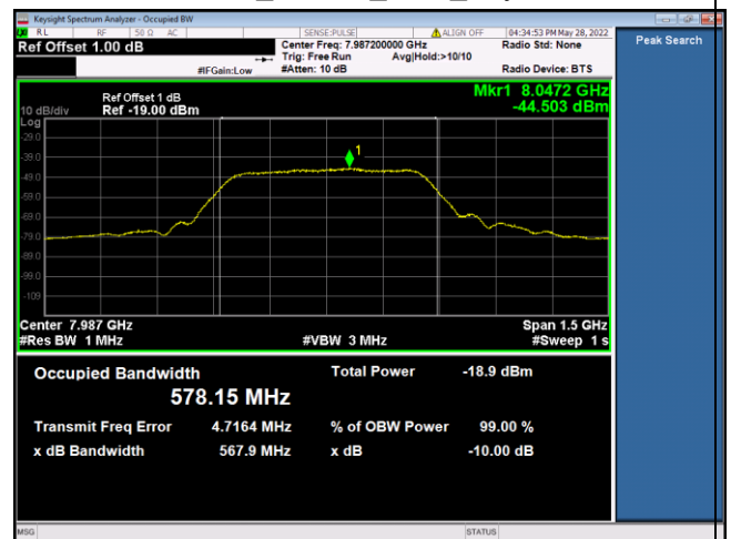
7987.2MHz_HPRF1_SP 1_STS 1_Payload 2
