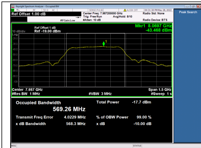
7987.2MHz_BPRF_SP 3_STS 2_Payload 0
