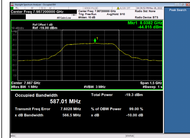
7987.2MHz_HPRF2_SP 1_STS 1_Payload 512
