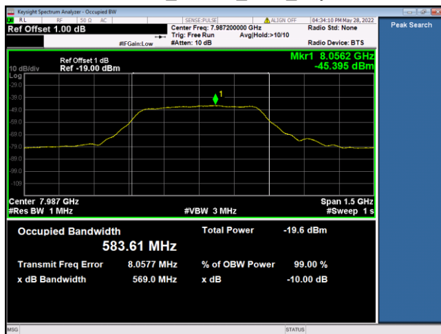
7987.2MHz_HPRF1_SP 0_Payload 1023
