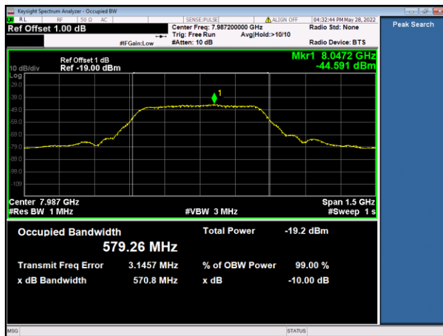
7987.2MHz_HPRF1_SP 0_Payload 2
