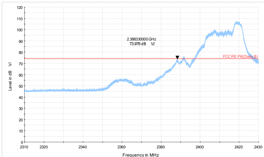
2.4G WIFI_ax20 CH1_2.31-2.43GHz_TP15.5_Y_52TONE_INDEX40_PK
