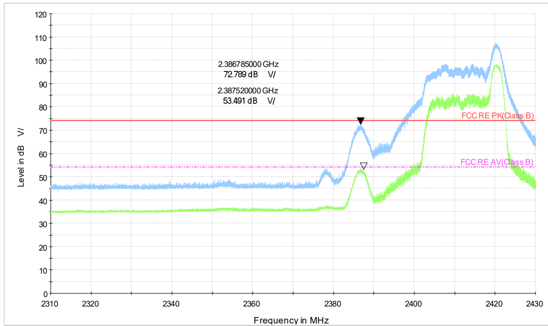
2.4G WIFI_ax20 CH1_2.31-2.43GHz_TP13_Y_26TONE_INDEX8
