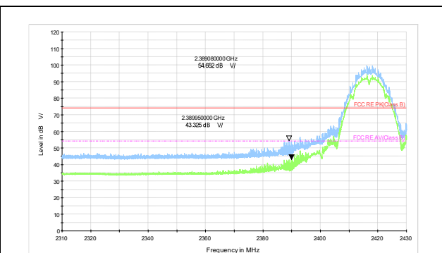
802.11b-Channel 2 Peak+ Average
