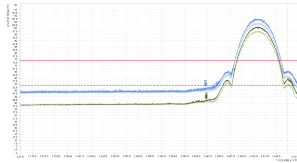
802.11ax HE20-Channel 1 Peak+ Average
