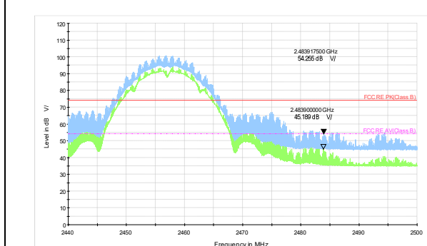
802.11b-Channel 10 Peak+ Average
