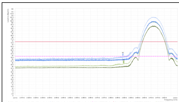
802.11b-Channel 1 Peak+ Average
