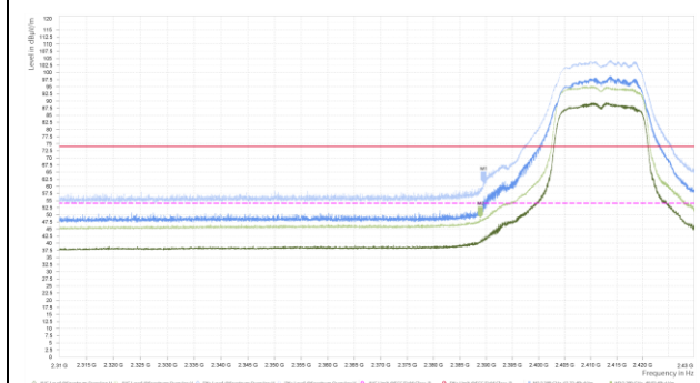
802.11g-Channel 1 Peak+ Average
