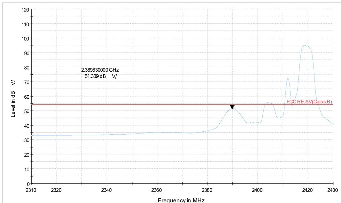
2.4G WIFI_ax20 CH1_2.31-2.43GHz_TP15.5_Y_52TONE_INDEX40_AV
