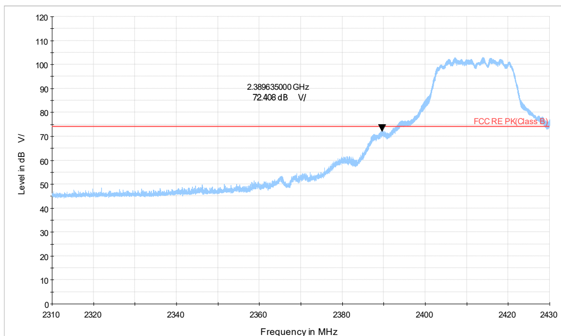
2.4G WIFI_ax20 CH1_2.31-2.43GHz_TP16.5_Y_242TONE_INDEX61_PK
