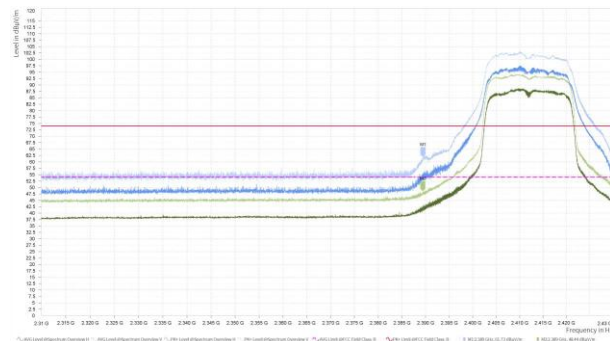
802.11n HT20-Channel 1 Peak+ Average
