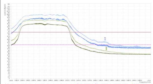
802.11g-Channel 11 Peak+ Average
