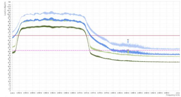
802.11ax HE20-Channel 11 Peak+ Average
