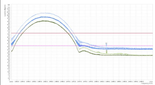
802.11b-Channel 11 Peak+ Average
