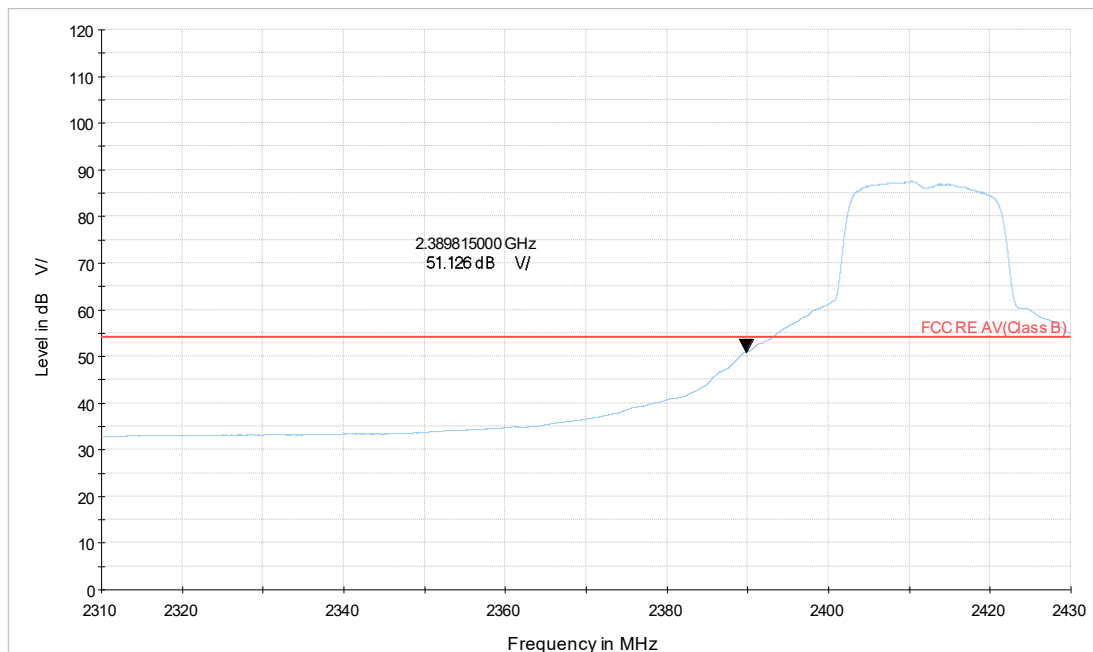
2.4G WIFI_ax20 CH1_2.31-2.43GHz_TP16.5_Y_242TONE_INDEX61_AV
