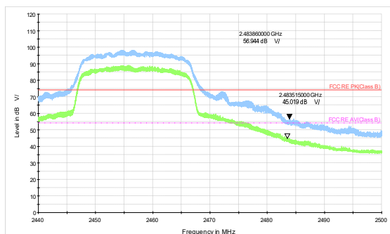
802.11ax HE20-Channel 10 Peak+ Average
