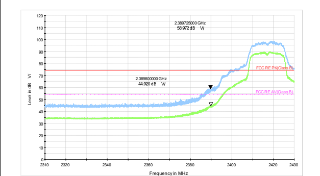
802.11g-Channel 2 Peak+ Average
