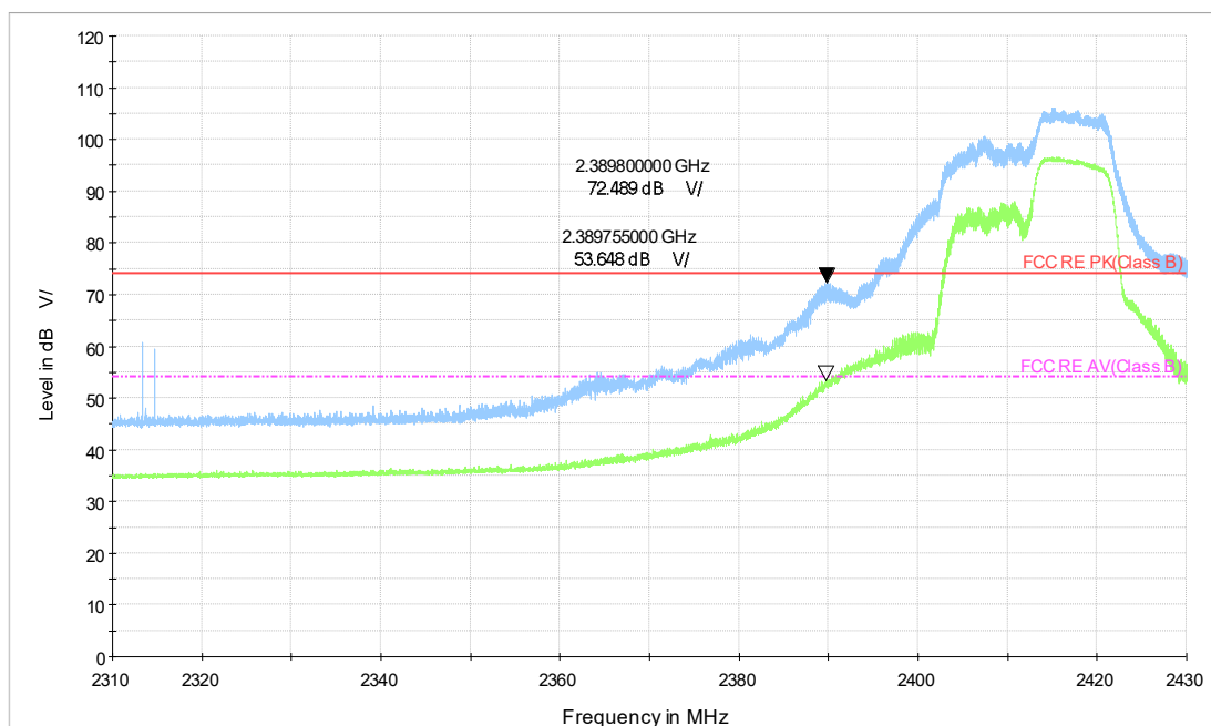
2.4G WIFI_ax20 CH1_2.31-2.43GHz_TP16.5_Y_106TONE_INDEX54
