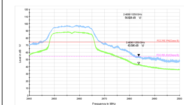
802.11g-Channel 10 Peak+ Average
