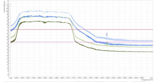
802.11n HT20-Channel 11 Peak+ Average
