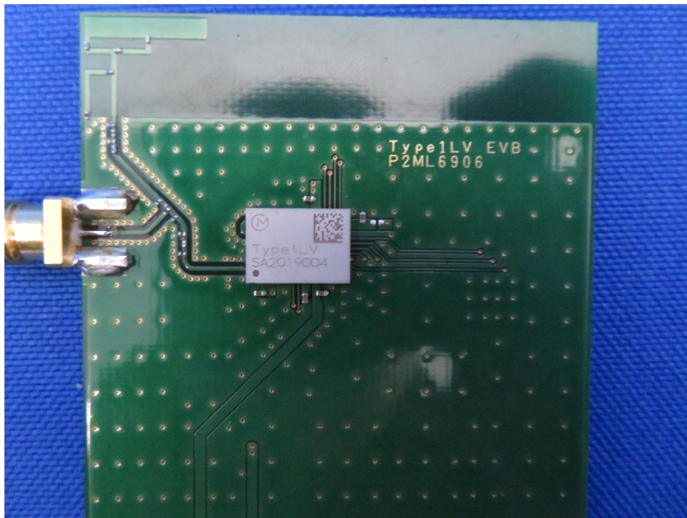
(3) EUT Photo (EUT + Test Fixture )
