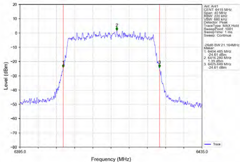
802.11ax(HE20)_HCH_6415MHz_RU242_Ant1_NTNV
