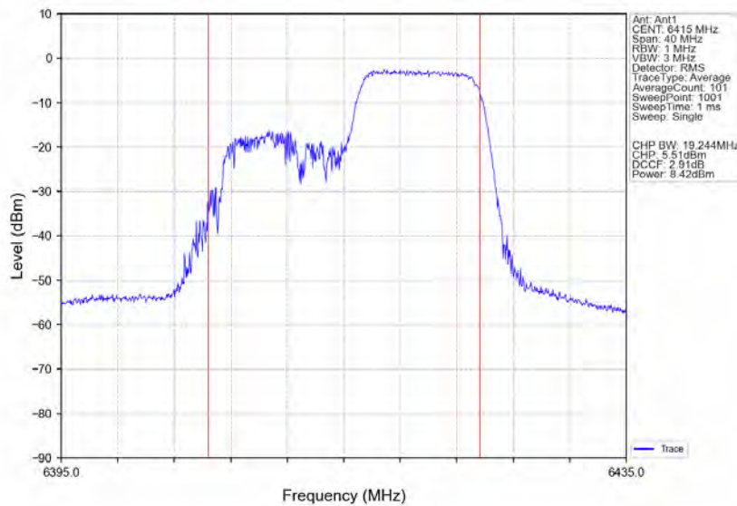
802.11ax(HE20)_HCH_6415MHz_RU106_Right_Ant1_NTNV
