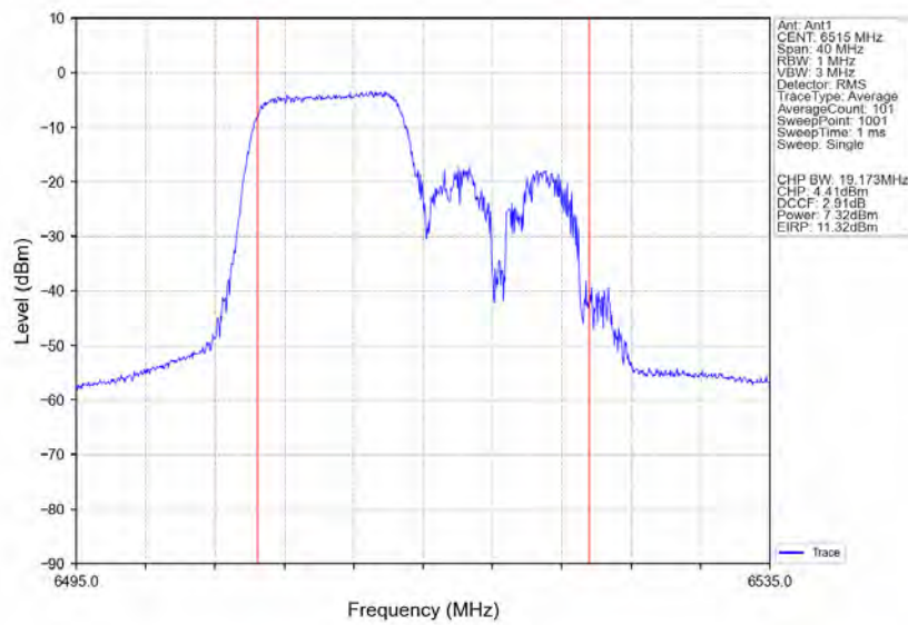
802.11ax(HE20)_HCH_6515MHz_RU106_Right_Ant1_NTNV
