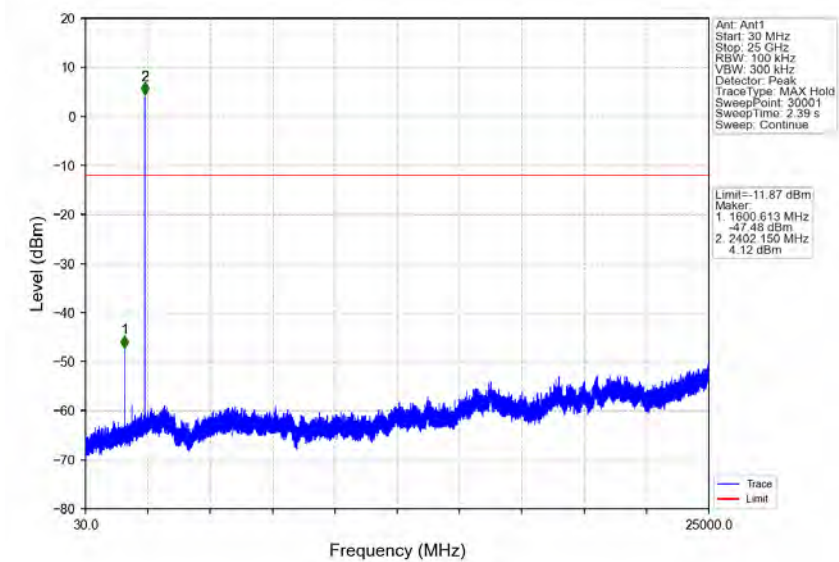
1M_LCH_2402MHz_Ant1_NTNV
