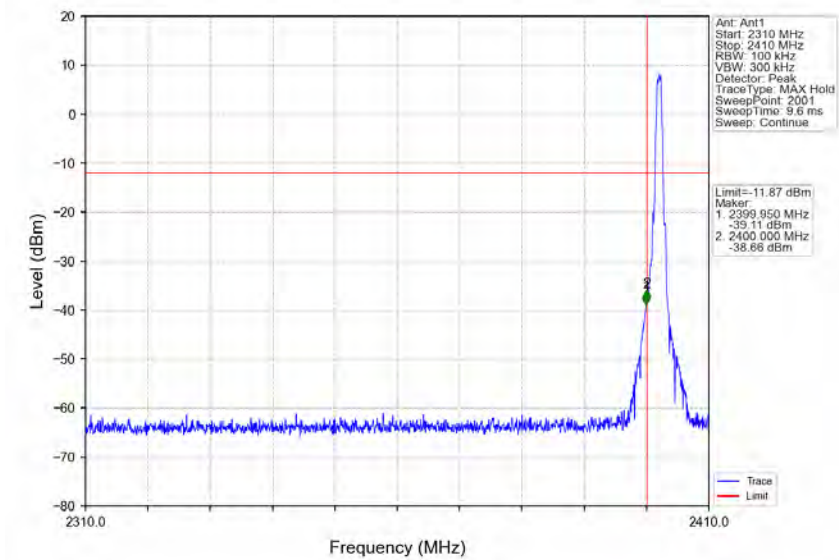
1M_LCH_2402MHz_Ant1_NTNV
