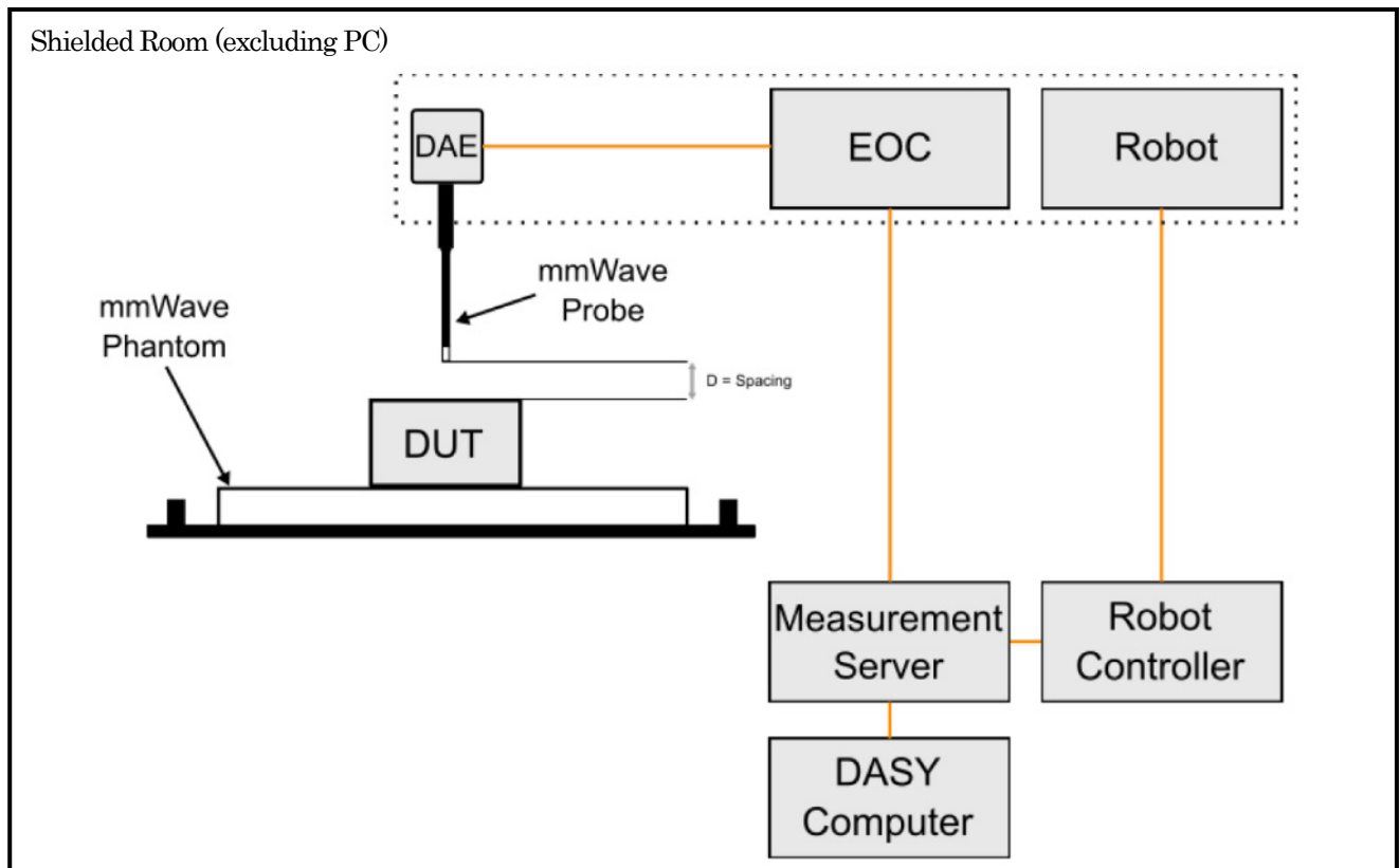
Figure 2-2 IPD Measurement System Description
