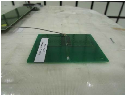
Monopole Antenna Axis X
