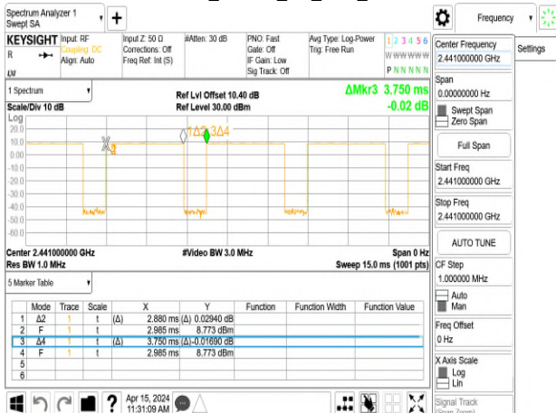
Dwell Time_8DPSK_3M_DH5_2441MHz
