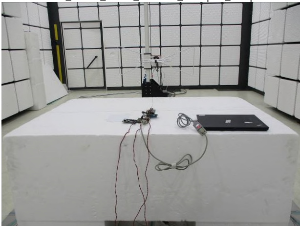
Part_15.247_WLAN_Radiated_monopole_Setup
