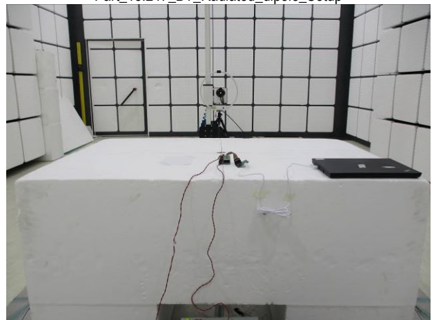
Part_15.247_BT_Radiated_dipole_Setup
