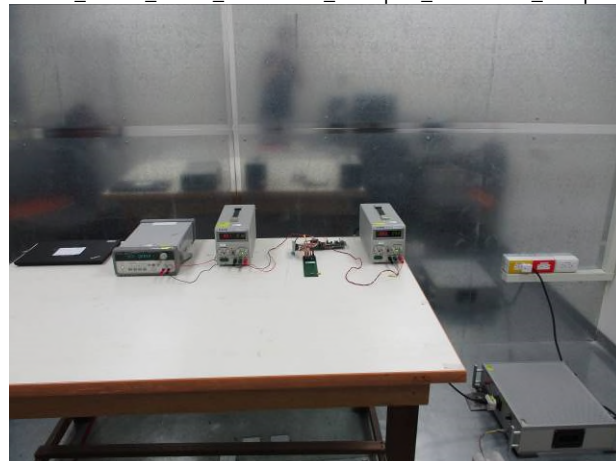
Part_15.247_WLAN_Conduction_monopole_Conduction_Setup
