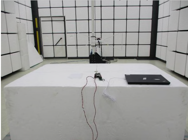
Part_15.247_LE_Radiated_dipole_Setup
