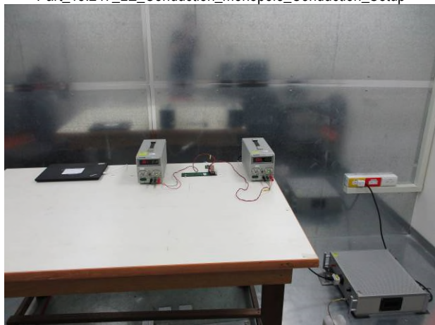
Part_15.247_LE_Conduction_monopole_Conduction_Setup
