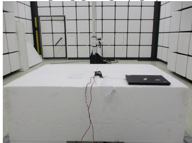
Part_15.247_LE_Radiated_monopole_Setup
