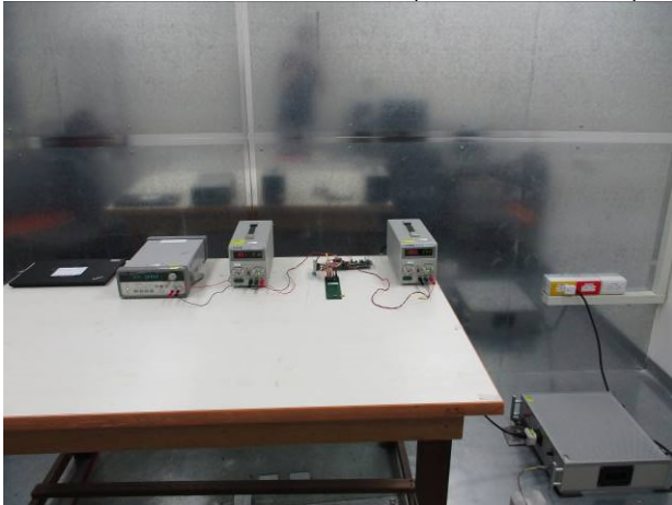
Part_15.407_WLAN_Conduction_monopole_Conduction_Setup
