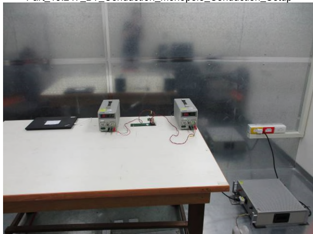
Part_15.247_BT_Conduction_monopole_Conduction_Setup
