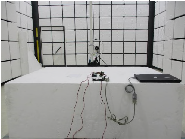
Part_15.407_WLAN_Radiated_dipole_Setup
