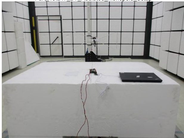
Part_15.247_BT_Radiated_monopole_Setup
