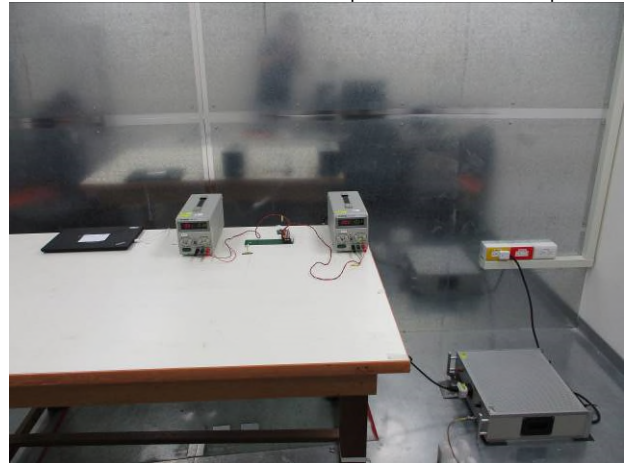
Part_15.247_LE_Conduction_dipole_Conduction_Setup
