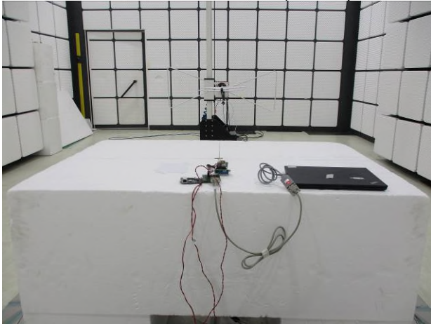
Part_15.247_WLAN_Radiated_dipole_Setup
