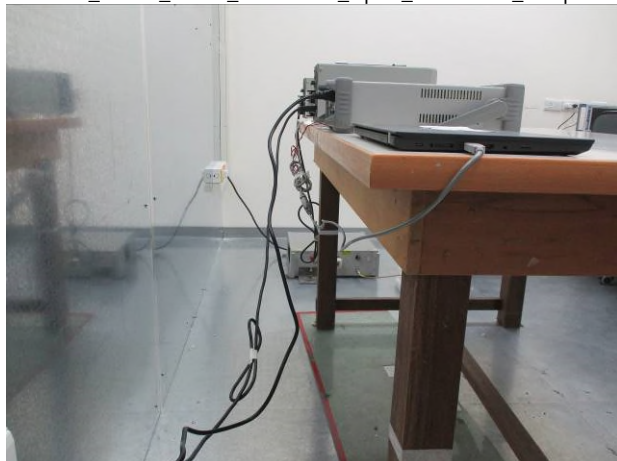
Part_15.407_WLAN_Conduction_dipole_Conduction_Setup
