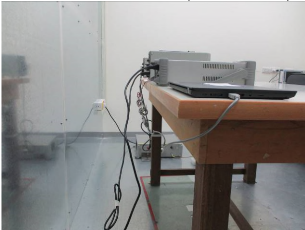
Part_15.247_BT_Conduction_dipole_Conduction_Setup
