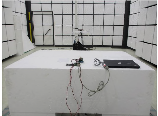
Part_15.407_WLAN_Radiated_dipole_Setup
