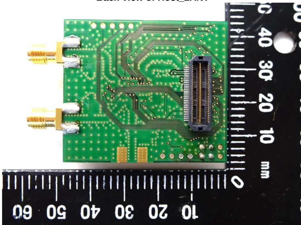
Back View of Host_2ANT
