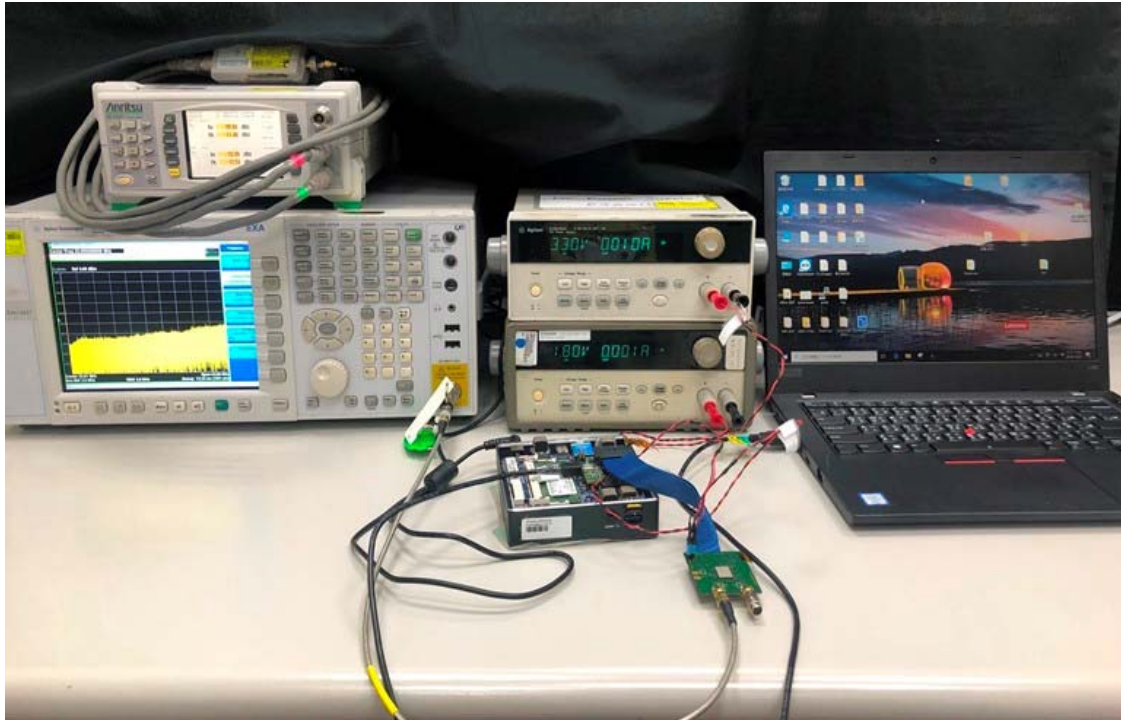
Conducted Setup Photo (Measurement at Antenna Port)_3ANT
