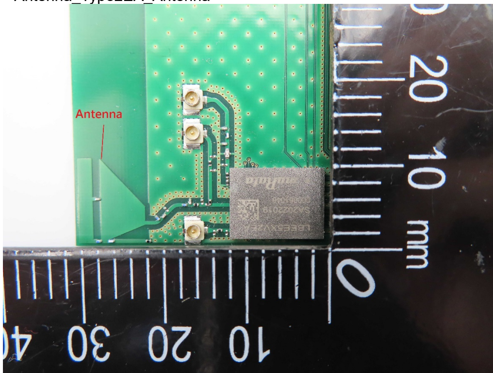
Antenna_Type2EA Antenna
