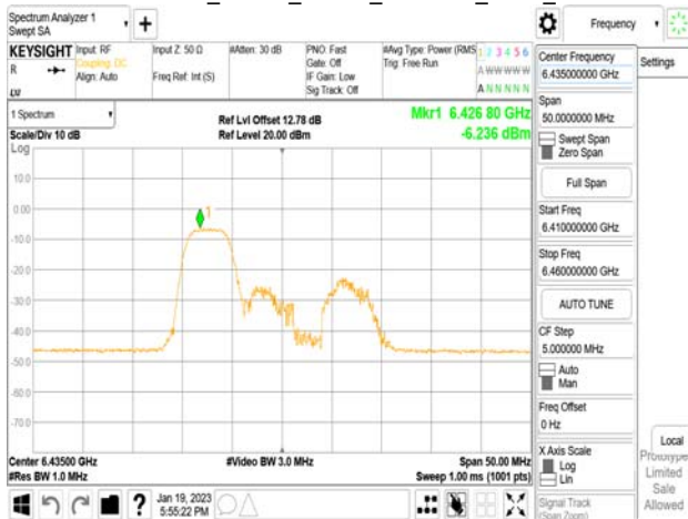
802.11ax_20MHz_Chain0_6435MHz_RU106_53
