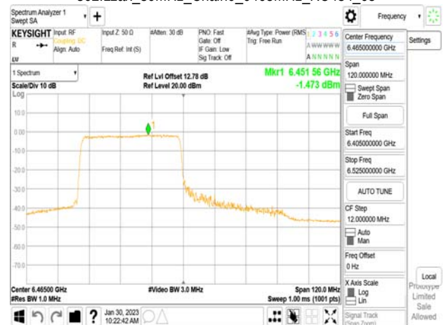
802.11ax_80MHz_Chain0_6465MHz_RU484_66
