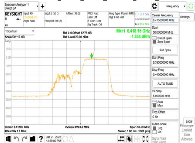
802.11ax_20MHz_Chain0_6415MHz_RU106_54
