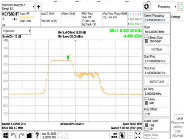
802.11ax_20MHz_Chain1_6435MHz_RU106_53
