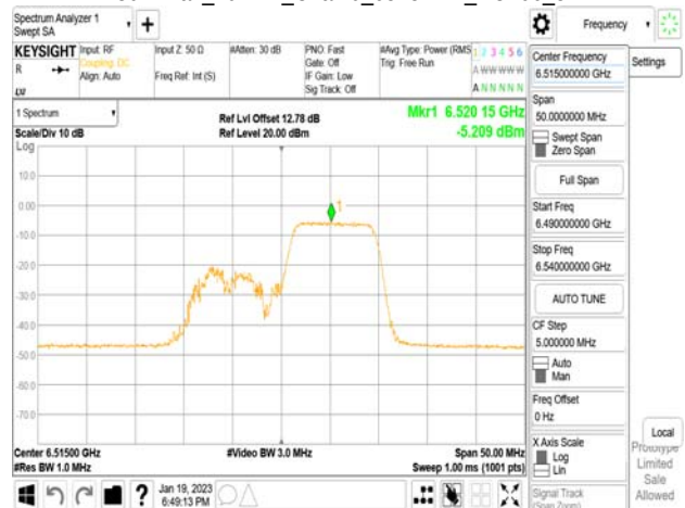
802.11ax_20MHz_Chain0_6515MHz_RU106_54
