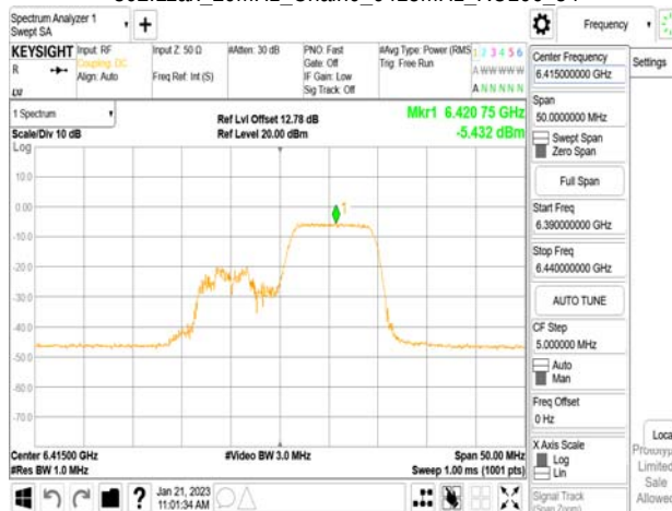
802.11ax_20MHz_Chain0_6415MHz_RU106_54
