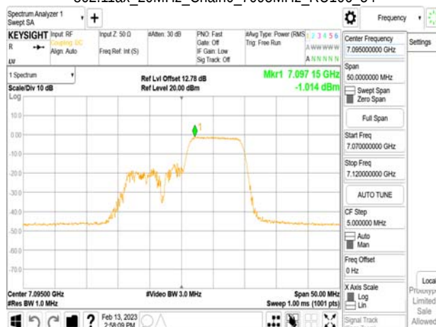
802.11ax_20MHz_Chain0_7095MHz_RU106_54
