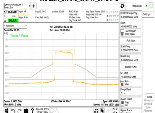
802.11ax_80MHz_Chain0_6545MHz
