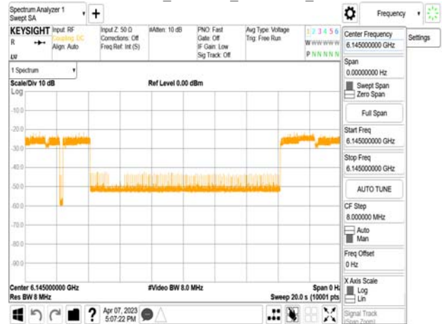
802.11ax_80MHz_CF 6145MHz_ Interference_6145MHz_-71.15dBm_Minimal
