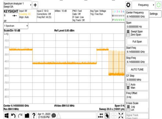
802.11ax_80MHz_CF 6145MHz_ Interference_6145MHz_-70.56dBm_Minimal
