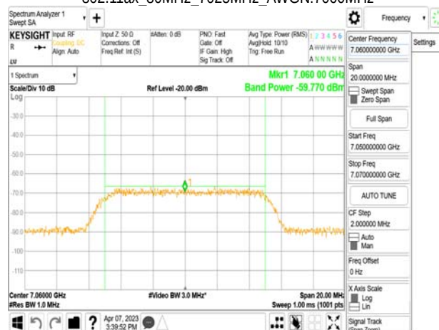
802.11ax_80MHz_7025MHz_AWGN:7060MHz
