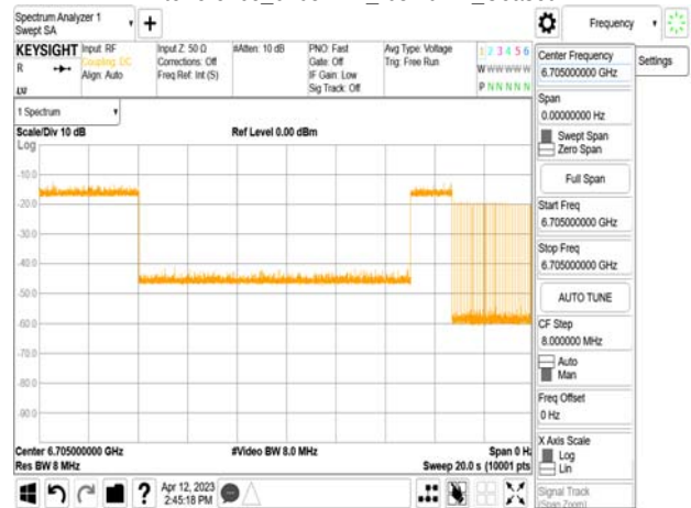
802.11ax_80MHz_CF 6705MHz_ Interference_6705MHz_-71.7dBm_Minimal
