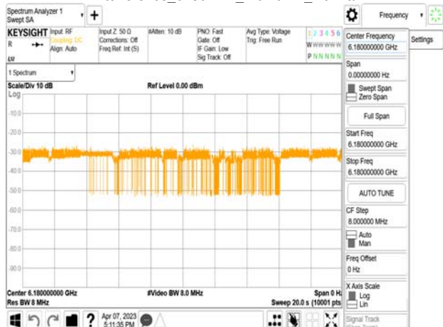
802.11ax_80MHz_CF 6145MHz_ Interference_6180MHz_-70.7dBm_Normal
