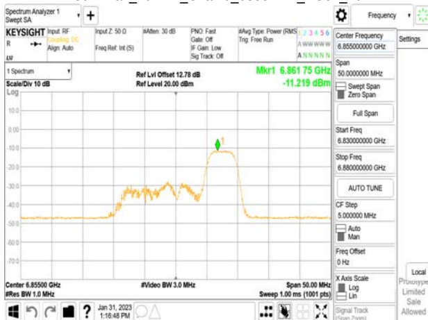
802.11ax_20MHz_Chain0_6855MHz_RU106_54
