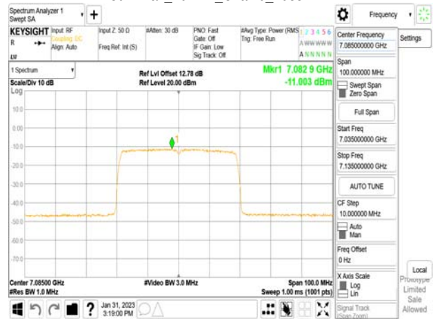
802.11ax_40MHz_Chain0_7085MHz_RU242_62
