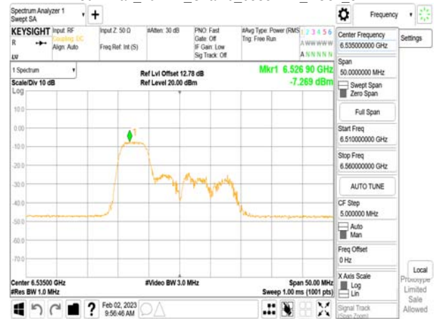
802.11ax_20MHz_Chain0_6535MHz_RU106_53
