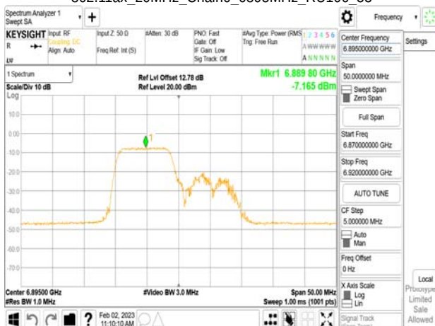
802.11ax_20MHz_Chain0_6895MHz_RU106_53
