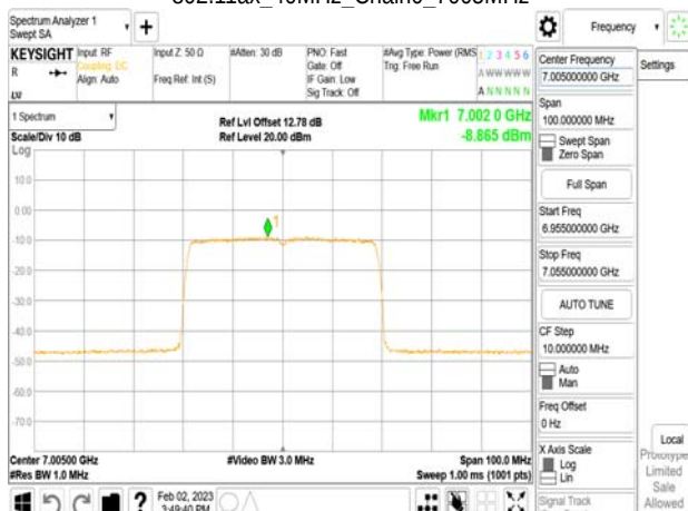
802.11ax_40MHz_Chain0_7005MHz
