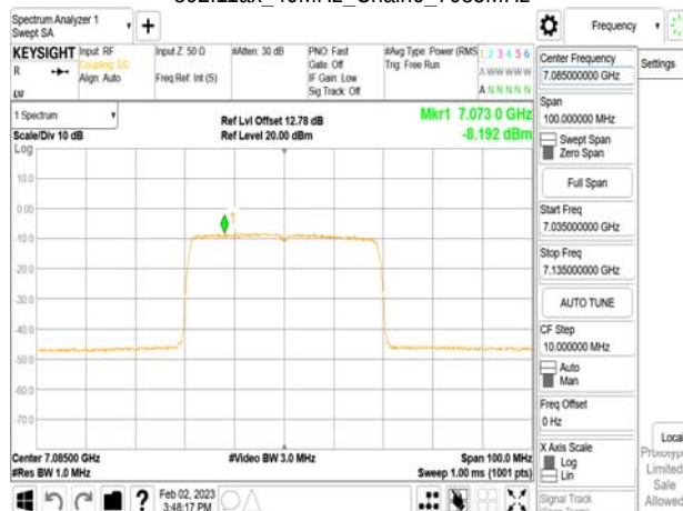
802.11ax_40MHz_Chain0_7085MHz_RU242_62
