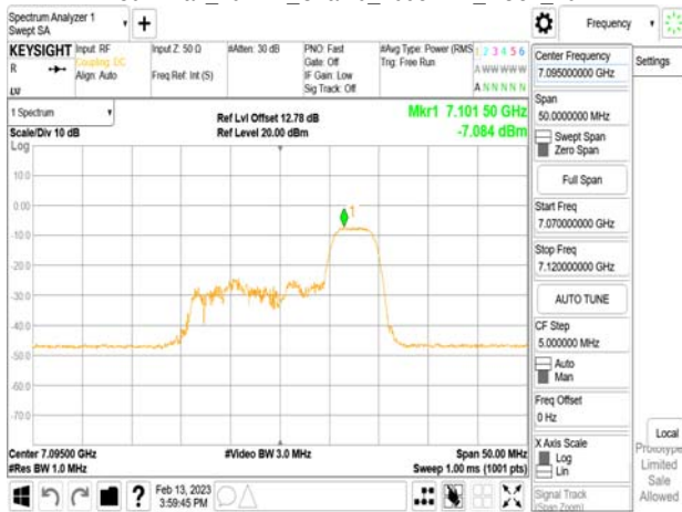
802.11ax_20MHz_Chain0_7095MHz_RU106_54
