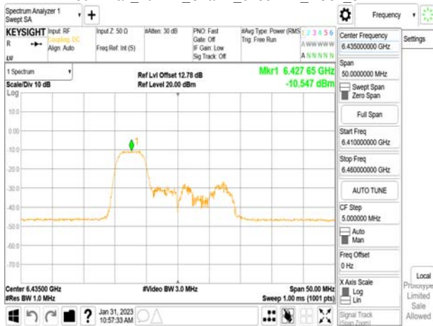
802.11ax_20MHz_Chain1_6435MHz_RU106_53
