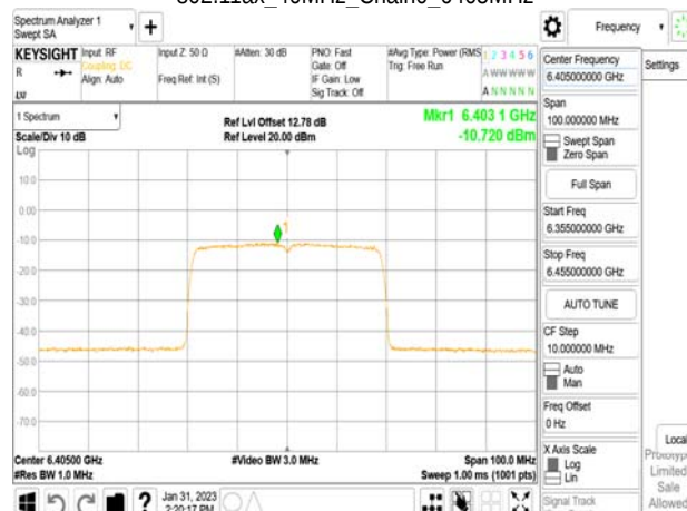
802.11ax_40MHz_Chain0_6405MHz
