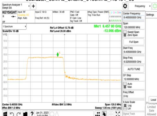
802.11ax_80MHz_Chain0_6465MHz_RU484_65
