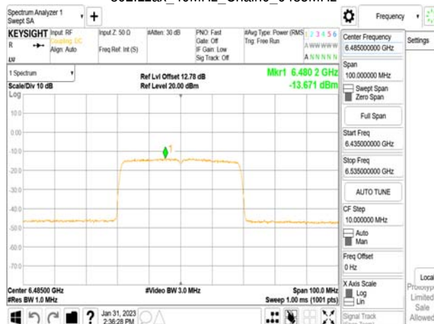
802.11ax_40MHz_Chain0_6485MHz_RU242_62
