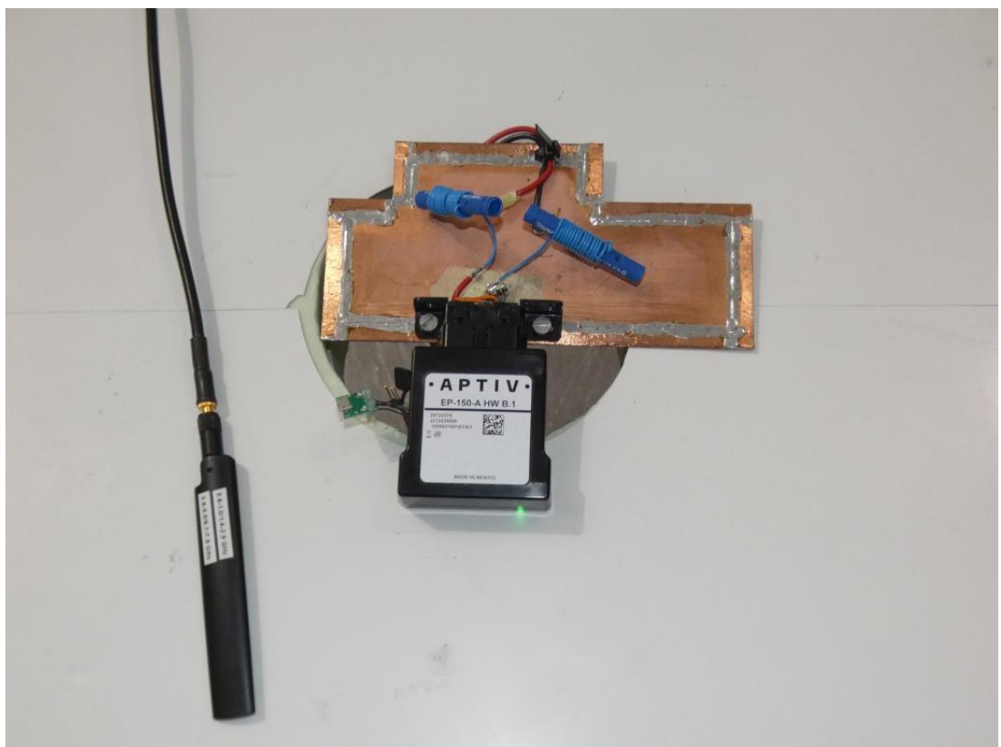
Photo 8: Test setup for radiated measurements EUT Detail
