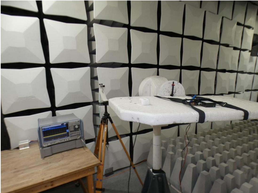
Photo 5: Test setup for radiated measurements above 26 GHz
