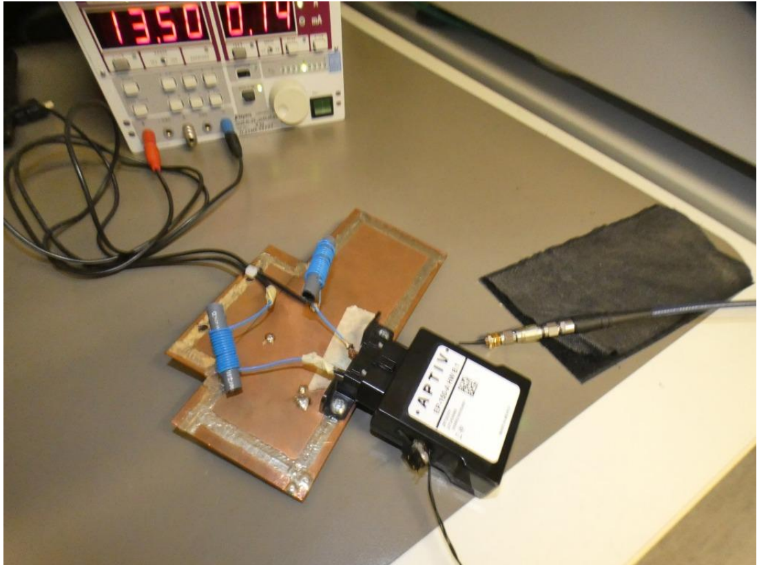
Photo 7: Test setup for conducted measurements EUT Detail
