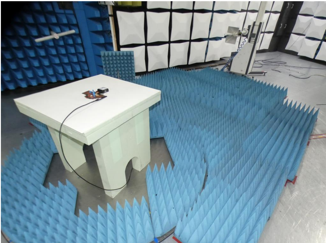
Photo 4: Test setup for radiated measurements 1 GHz to 18 GHz FCC 15b
