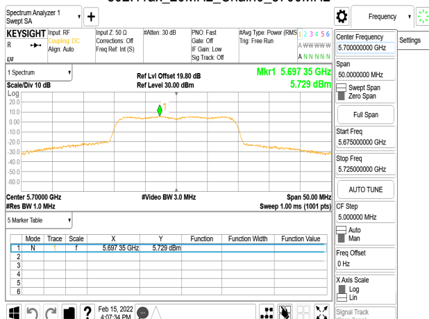
802.11ax_20MHz_Chain0_5700MHz_RU106_54
