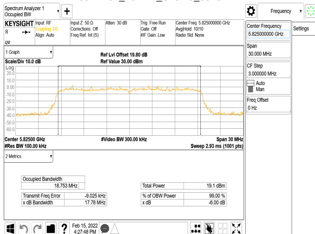
802.11ax_20MHz_Chain0_5825MHz_RU106_54
