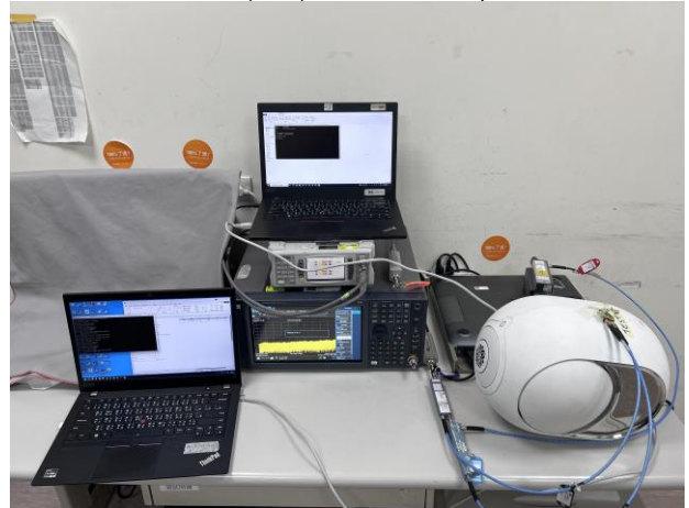
WLAN(5G)_Conducted_Setup-1
