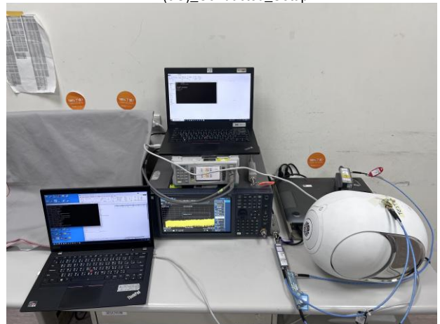
WLAN(5G)_Conducted_Setup-2
