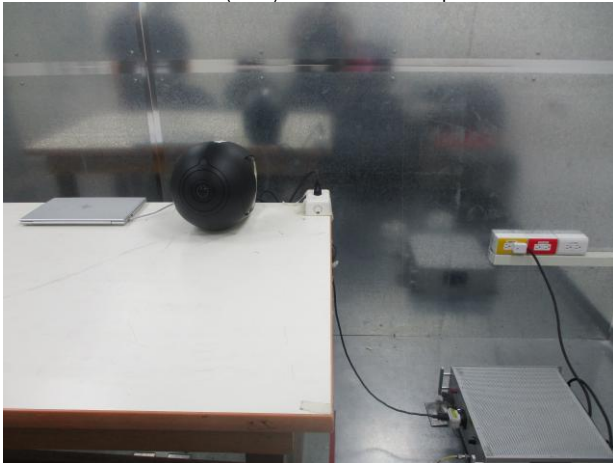
WLAN(2.4G)_Conduction_Setup
