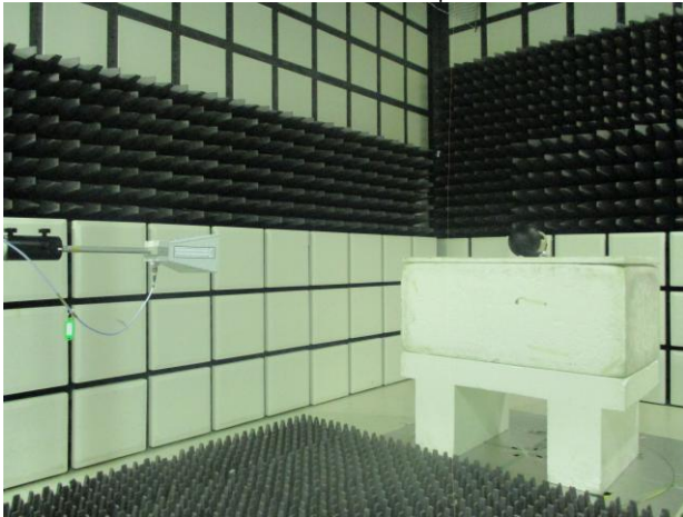
BLE_Radiated_Setup
