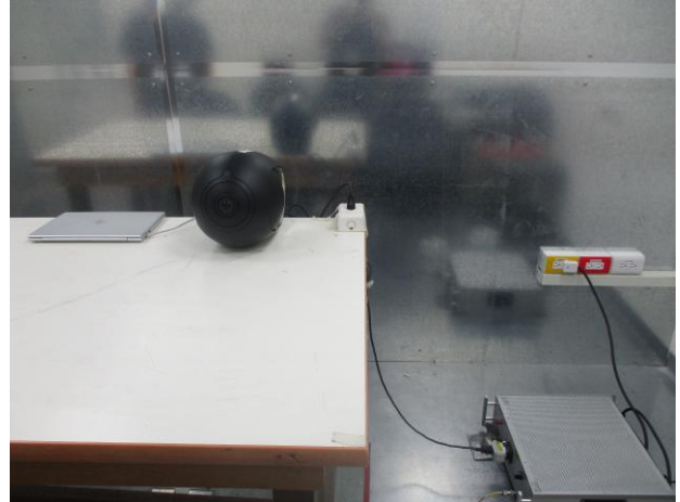
BLE_Conduction_Setup
