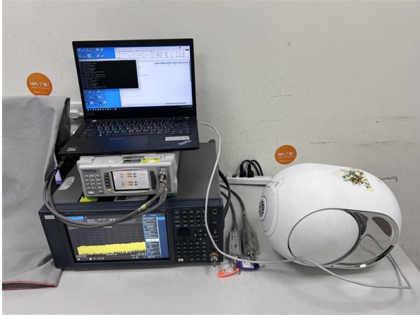
WLAN(2.4G)_Conducted_Setup-1
