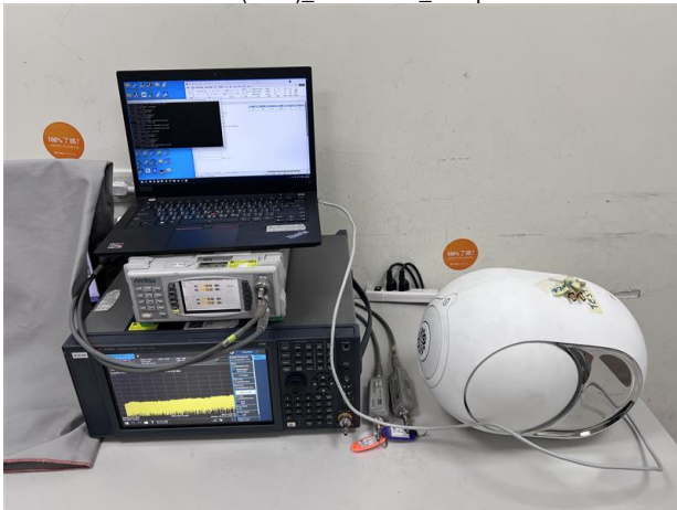
WLAN(2.4G)_Conducted_Setup-1
