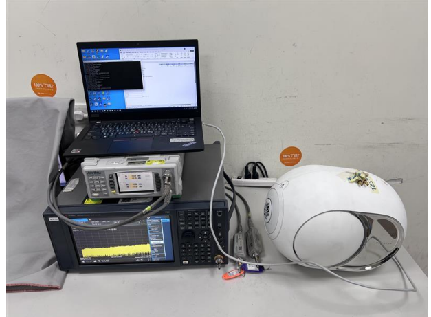
WLAN(5G)_Conducted_Setup-2
