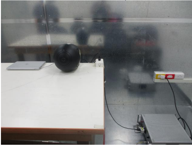
BT_Conduction_Setup
