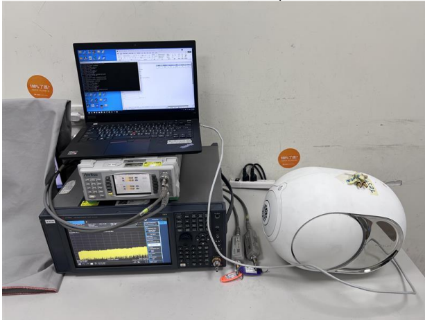
BT_Conducted_Setup
