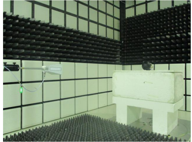
WLAN(2.4G)_Radiated_Setup
