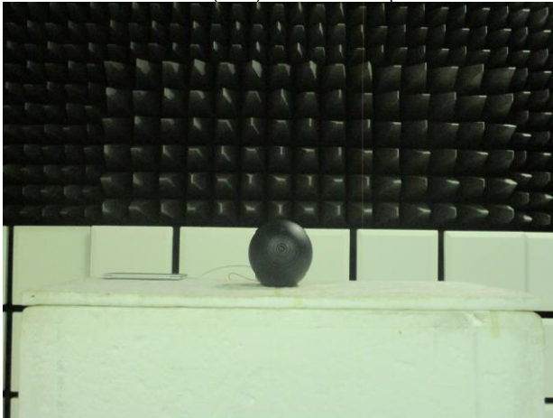
WLAN(2.4G)_Radiated_Setup
