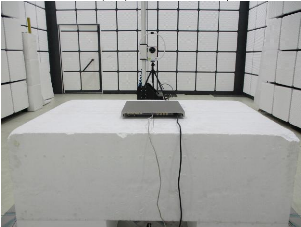
WLAN(5G)_Radiated_966D_Setup
