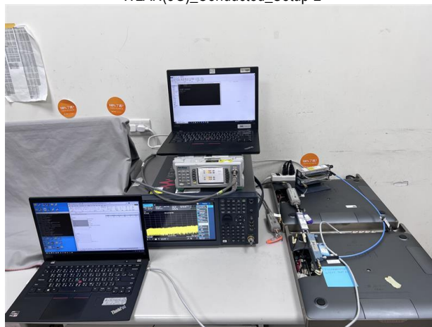
WLAN(5G)_Conducted_Setup-2
