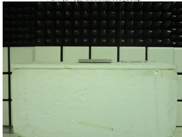
WLAN(2.4G)_Radiated_966G_Setup
