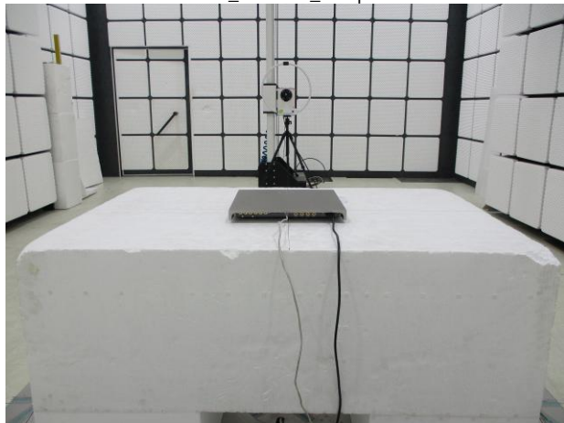
WLAN(2.4G)_Radiated_966D_Setup
