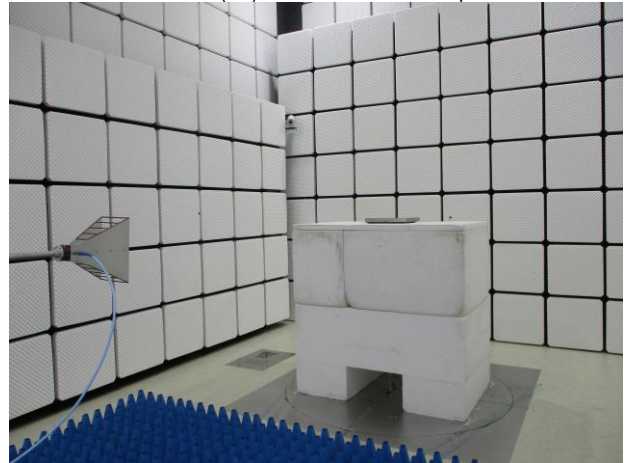
WLAN(5G)_Radiated_966G_Setup
