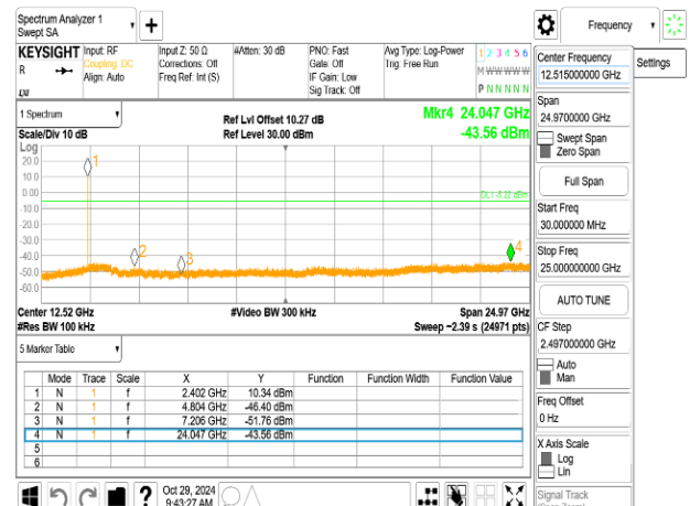
Spurious Emission_BLE 500k_LowCH00-2402MHz
