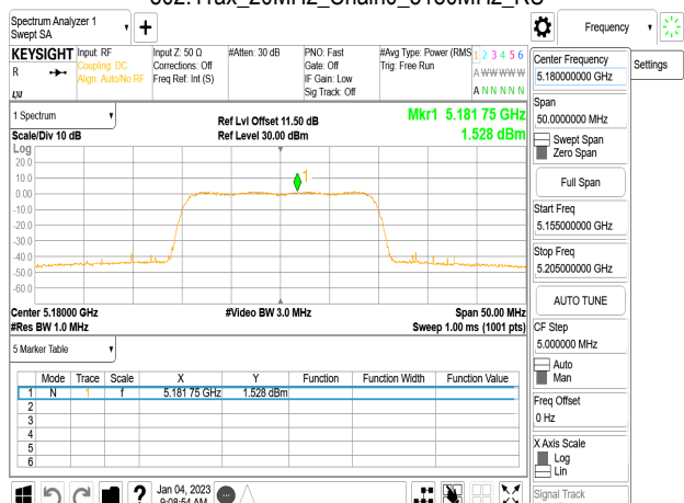
802.11ax_20MHz_Chain0_5180MHz_RU106_53
