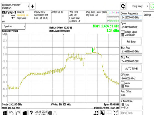
802.11ax_40MHz_Chain0_2422MHz_RU106_56
