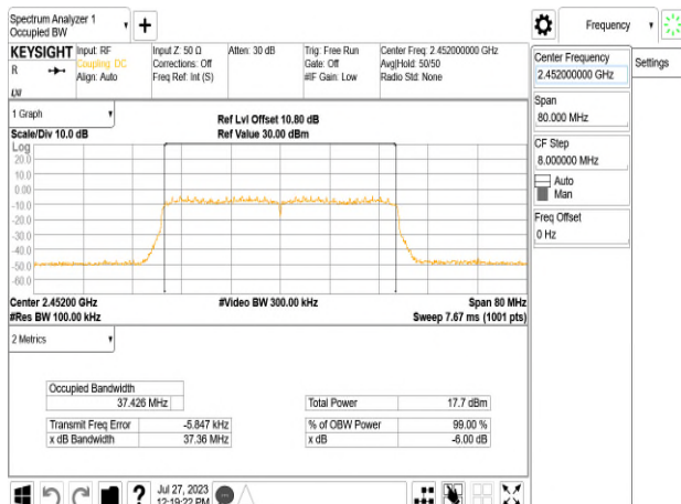
802.11ax_40MHz_Chain0_2452MHz
