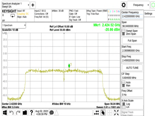
802.11ax_40MHz_Chain0_2422MHz_RU106_53
