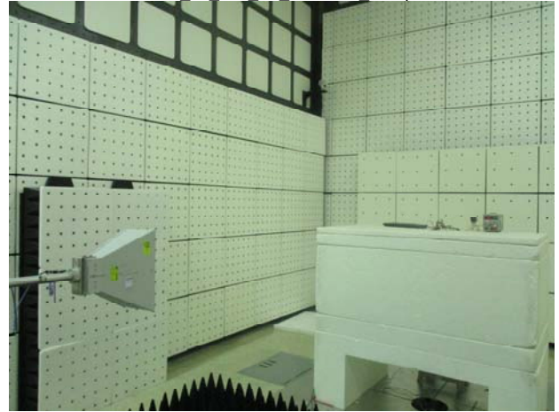
Part_15_247_LE_Radiated_Setup
