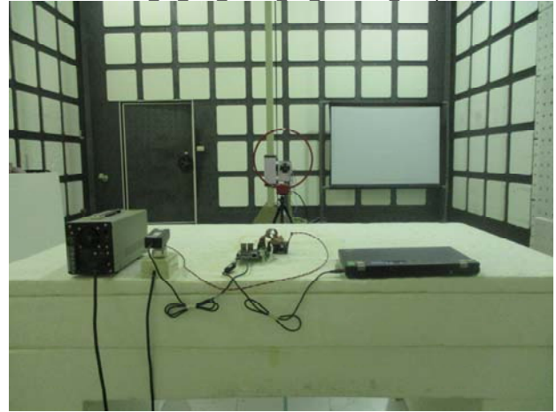
Part 15 407 WLAN 5G Conduction Setup
