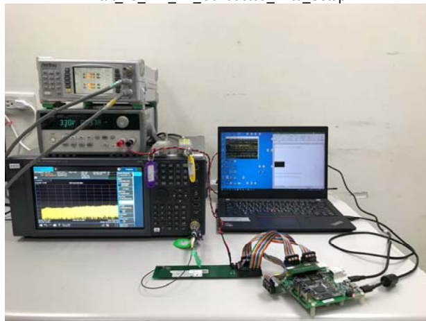
Part_15_247_BT_Conducted_Ant1_Setup
