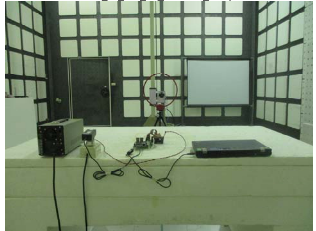
Part_15_247_LE_Radiated_Setup
