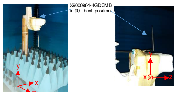
Antenna measured in Free Space
