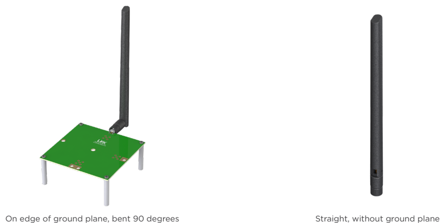
Figure 2. ANT-915-IPW1-RPS Antenna on Evaluation PCB
