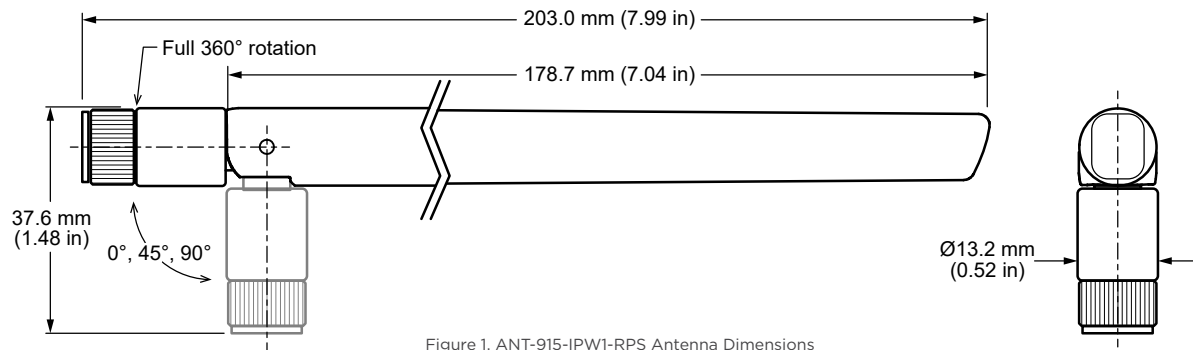
Figure 1. ANT-915-IPW1-RPS Antenna Dimensions
