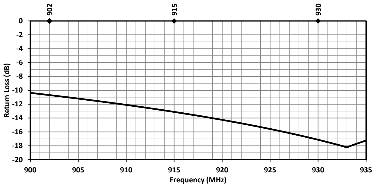
Figure 5. ANT-915-IPW1-RPS Antenna Return Loss, Edge Bent
