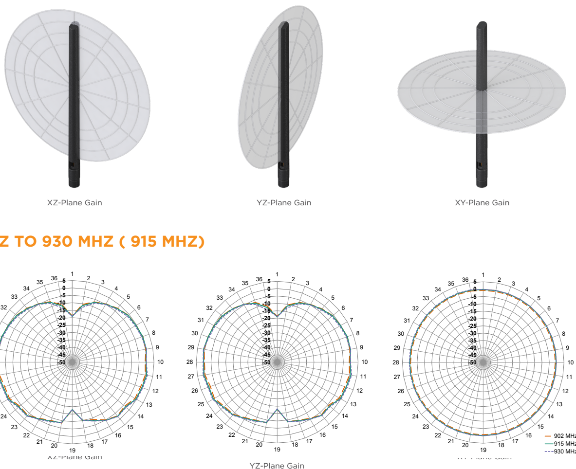
Figure 16. Radiation Patterns for ANT-915-IPW1-RPS, Straight
