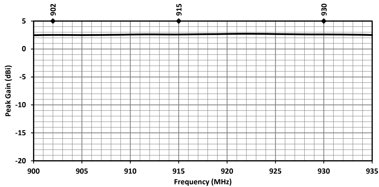
Figure 6. ANT-915-IPW1-RPS Antenna Peak Gain, Edge Bent
