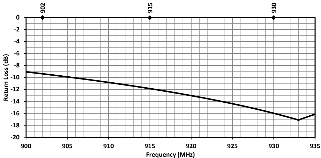
Figure 12. ANT-915-IPW1-RPS Antenna Return Loss, Straight
