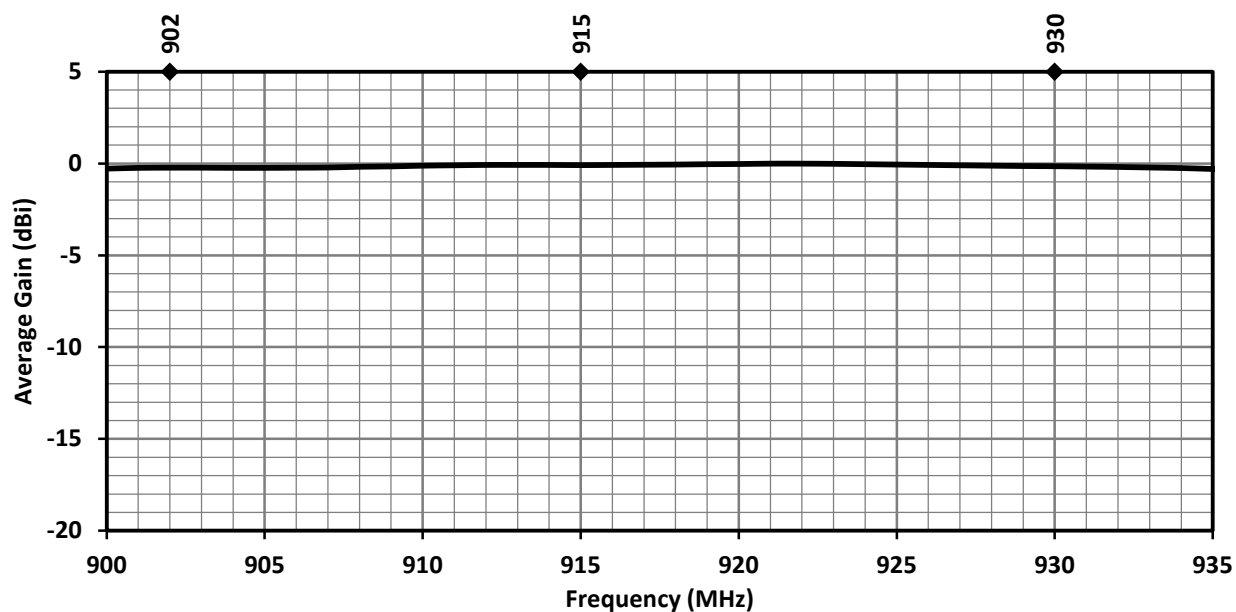
Figure 7. ANT-915-IPW1-RPS Antenna Average Gain, Edge Bent
