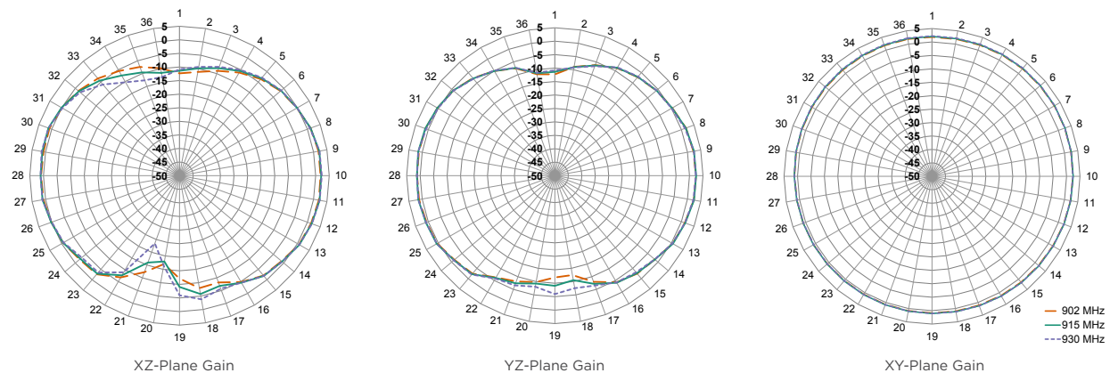
Figure 9. Radiation Patterns for ANT-915-IPW1-RPS, Edge Bent
