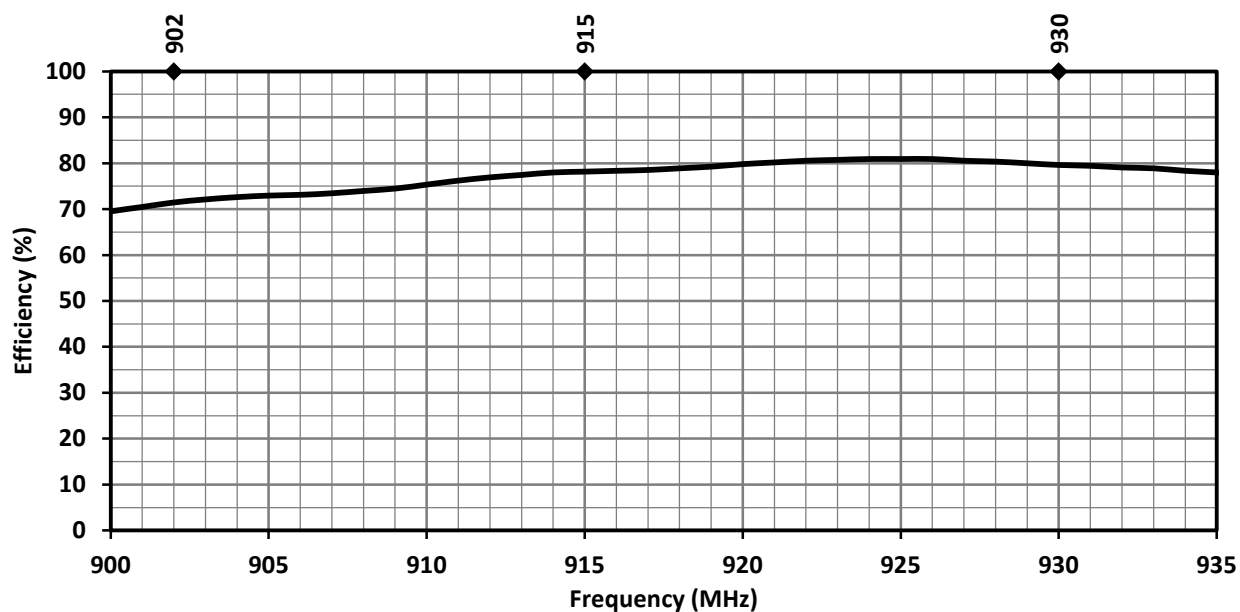
Figure 15. ANT-915-IPW1-RPS Antenna Radiation Efficiency, Straight
