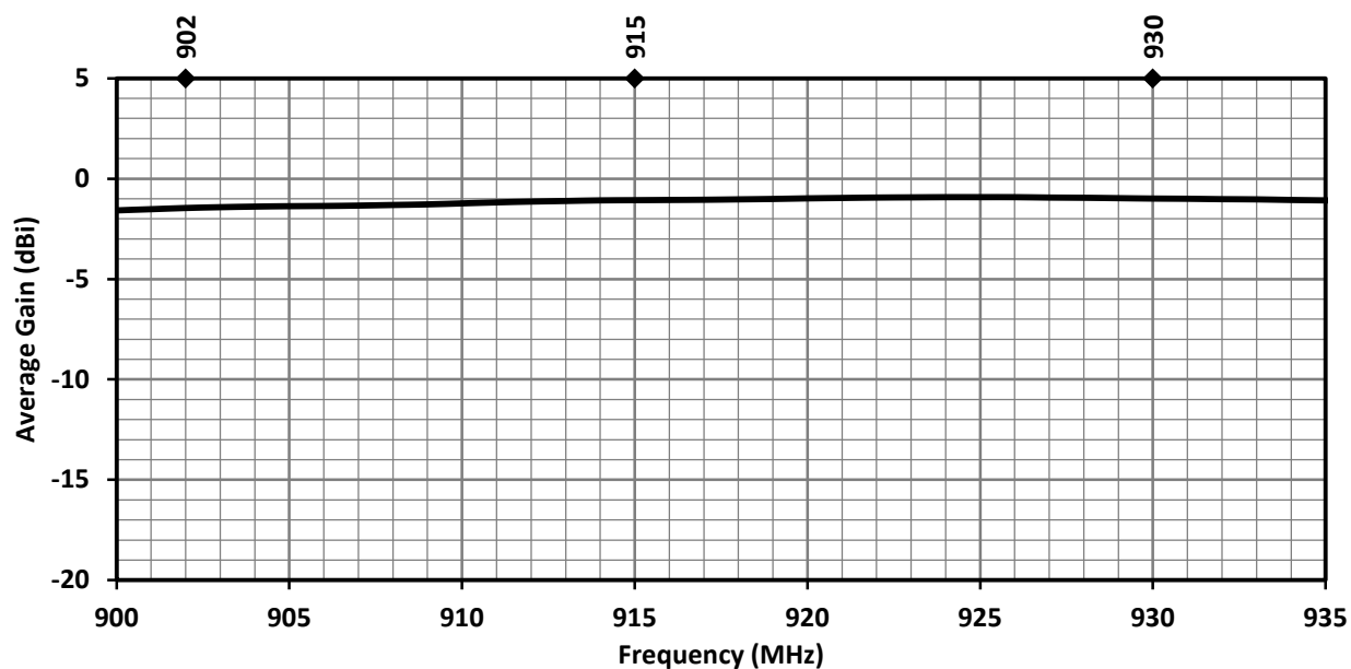
Figure 14. ANT-915-IPW1-RPS Antenna Average Gain, Straight
