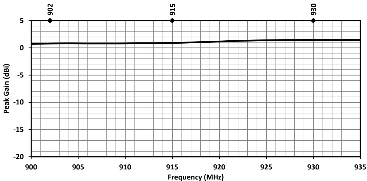
Figure 13. ANT-915-IPW1-RPS Antenna Peak Gain, Straight
