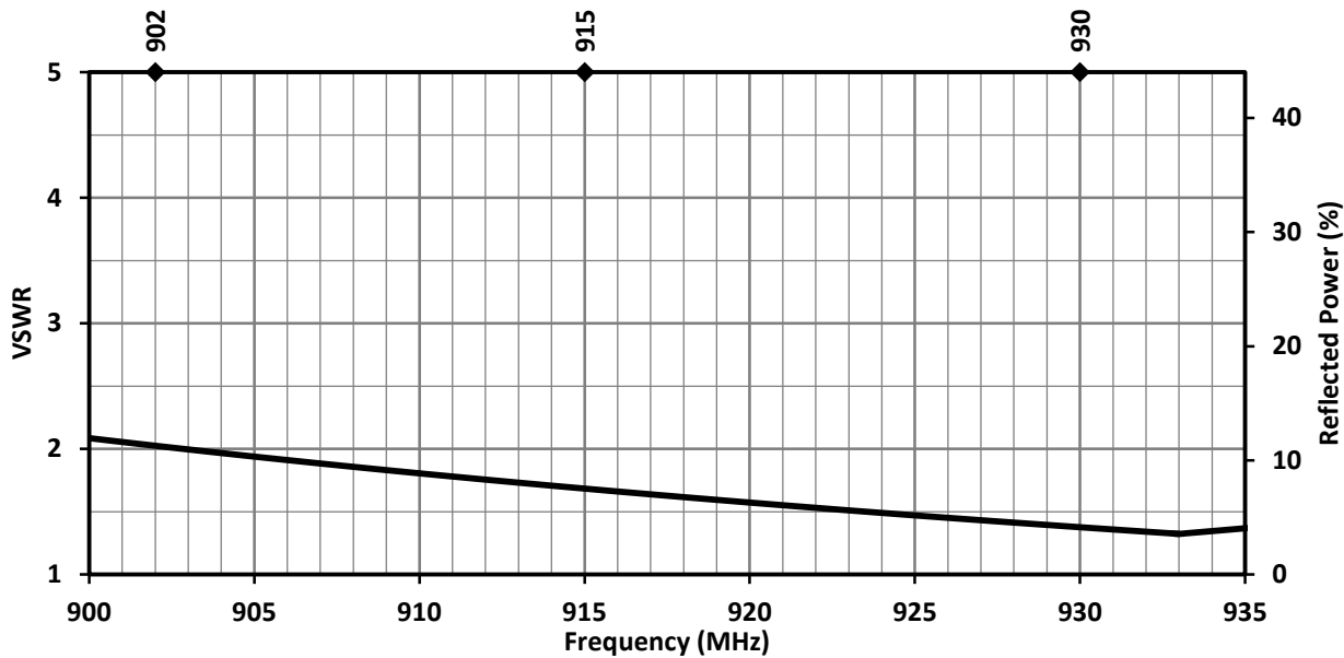
Figure 11. ANT-915-IPW1-RPS Antenna VSWR, Straight
