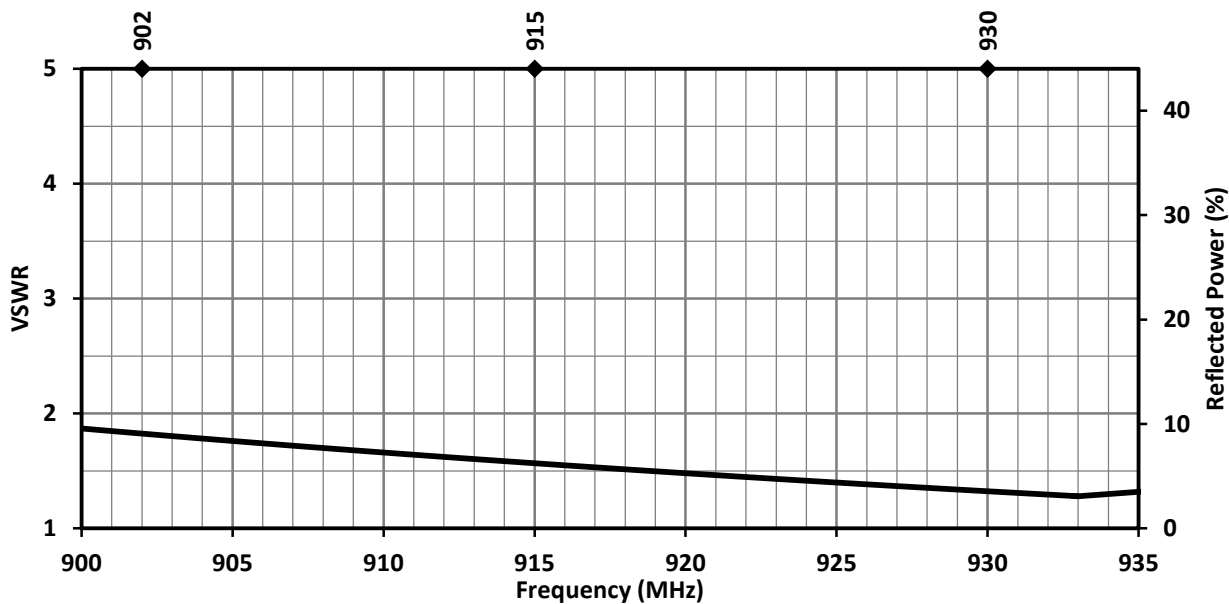
Figure 4. ANT-915-IPW1-RPS Antenna VSWR, Edge Bent
