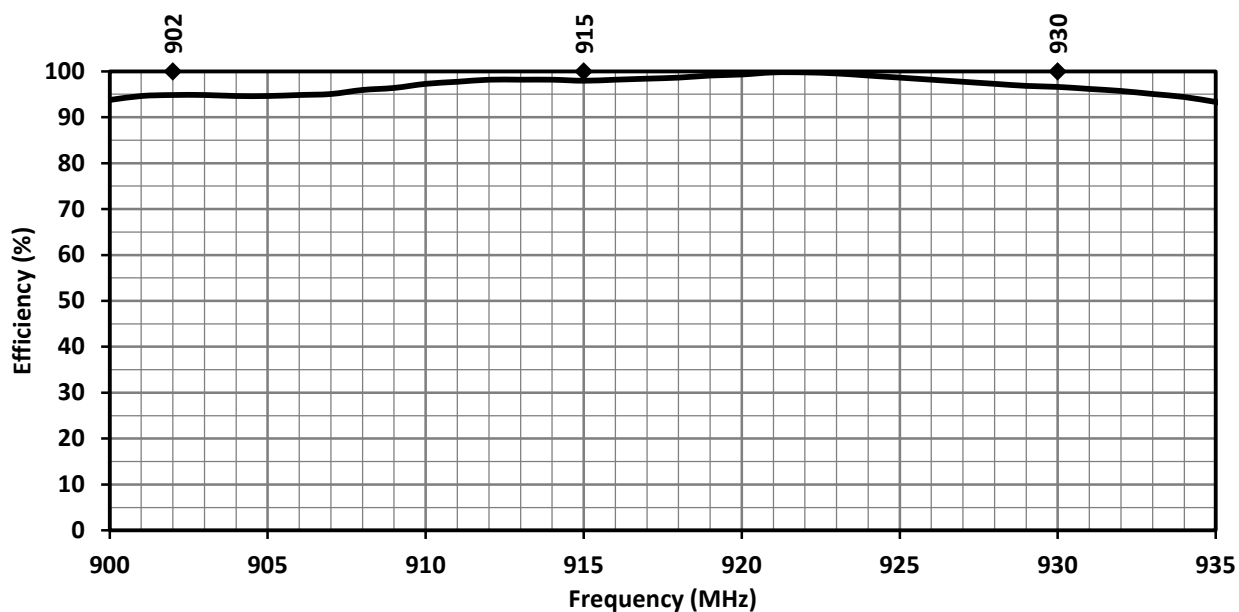
Figure 8. ANT-915-IPW1-RPS Antenna Radiation Efficiency, Edge Bent
