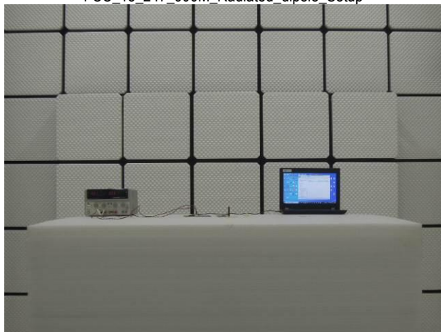
FCC_15_247_900M_Radiated_dipole_Setup
