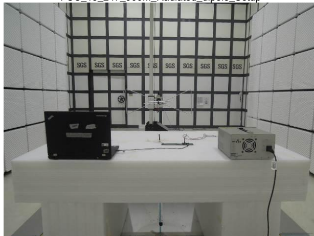
FCC_15_247_900M_Radiated_dipole_Setup
