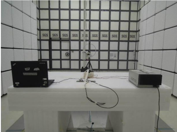
FCC_15_247_900M_Radiated_monopole_Setup
