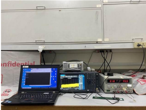
900MHz_Radiated_Setup
