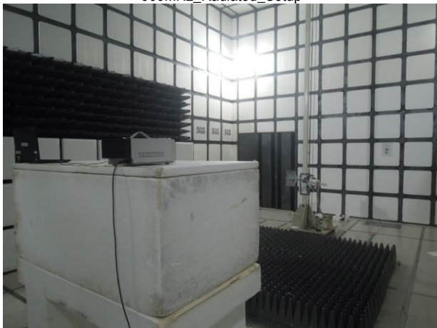
900MHz_Radiated_Setup
