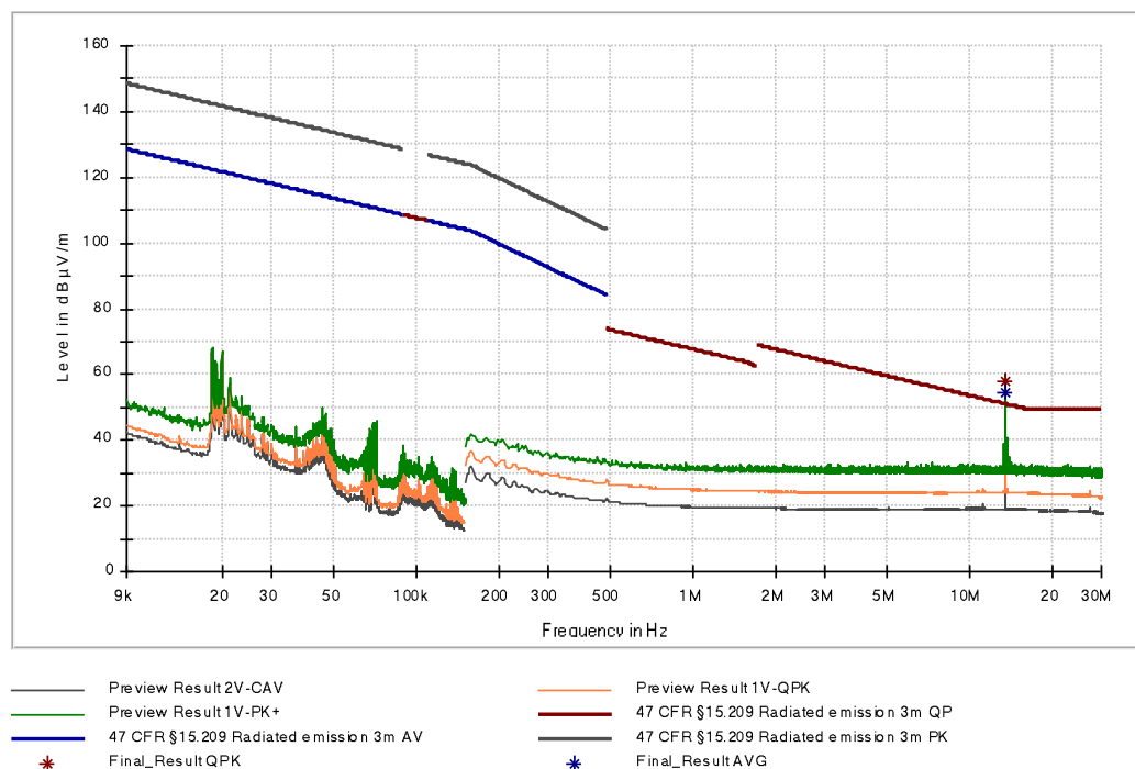
Figure 13: Chart of emissions test below 30 MHz without tag in position 2, antenna in line at 3 m
