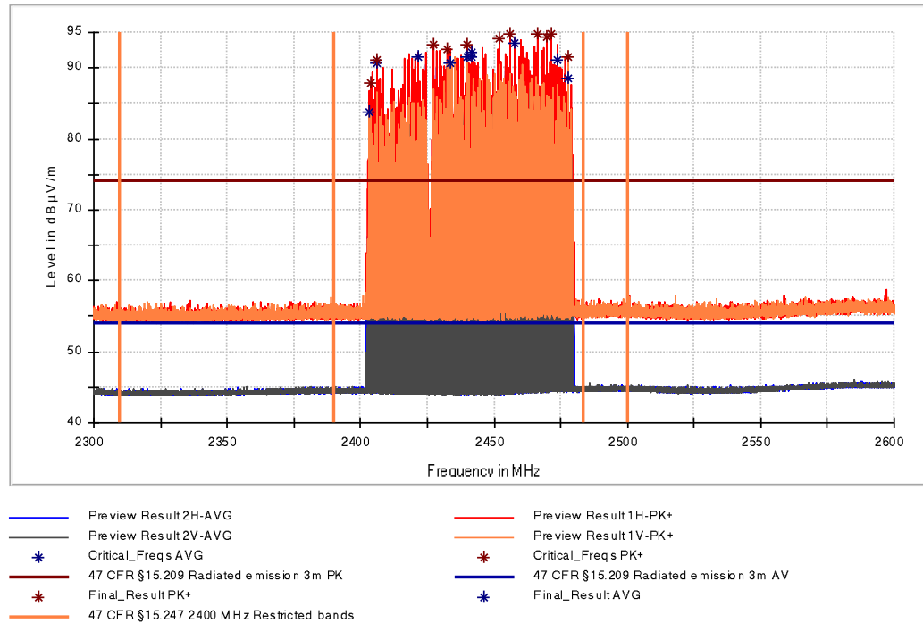
Figure 18: Chart of band-edge measurement
