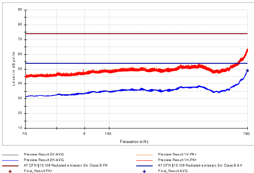
Figure 16: Chart of radiated disturbance test from 7 GHz to 18 GHz
