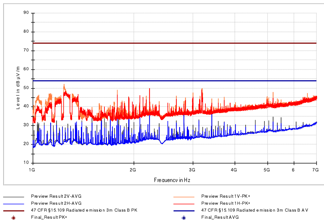
Figure 15: Chart of radiated disturbance test from 1 GHz to 7 GHz
