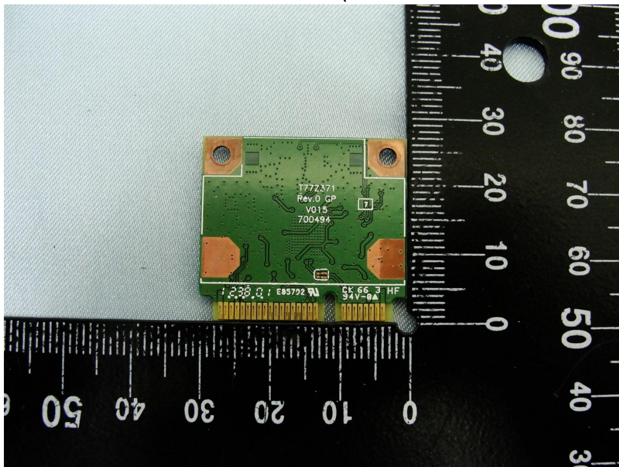
EUT: WLAN module (Brand Name: Ralink /Modle Name: RT3290)
