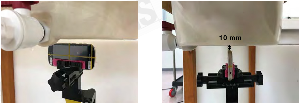
Fig.13 EUT Left side to flat phantom
