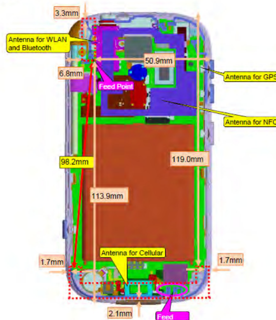
Fig.17 Antenna position of EUT
