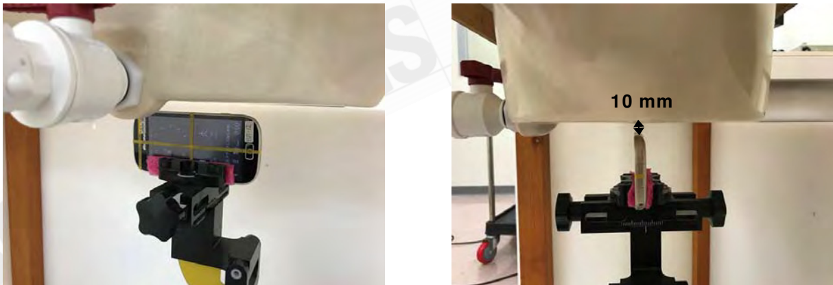
Fig.14 EUT Right side to flat phantom
