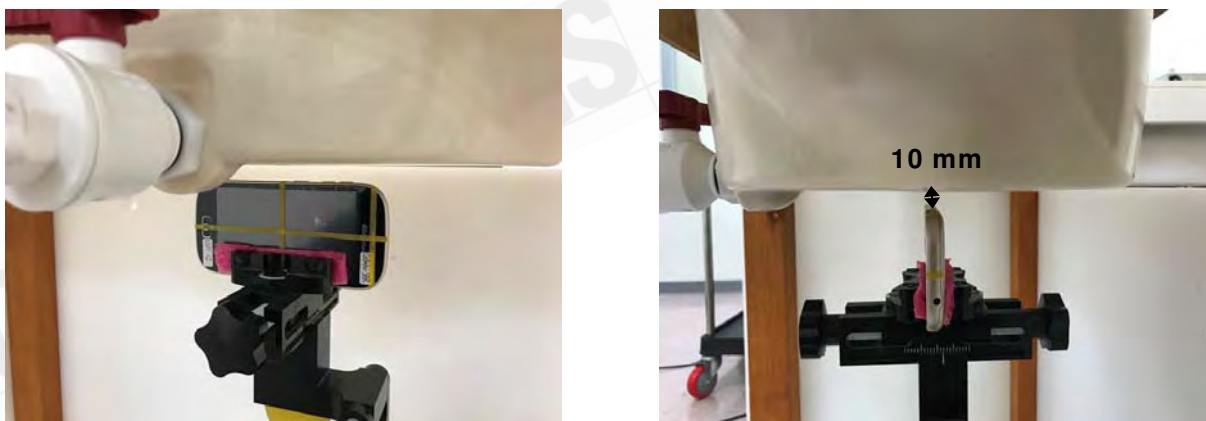
Fig.13 EUT Left side to flat phantom
