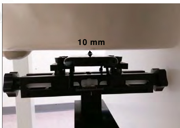
Fig.11 EUT Back side to flat phantom
