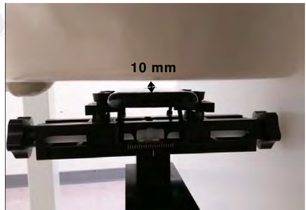
Fig.11 EUT Back side to flat phantom
