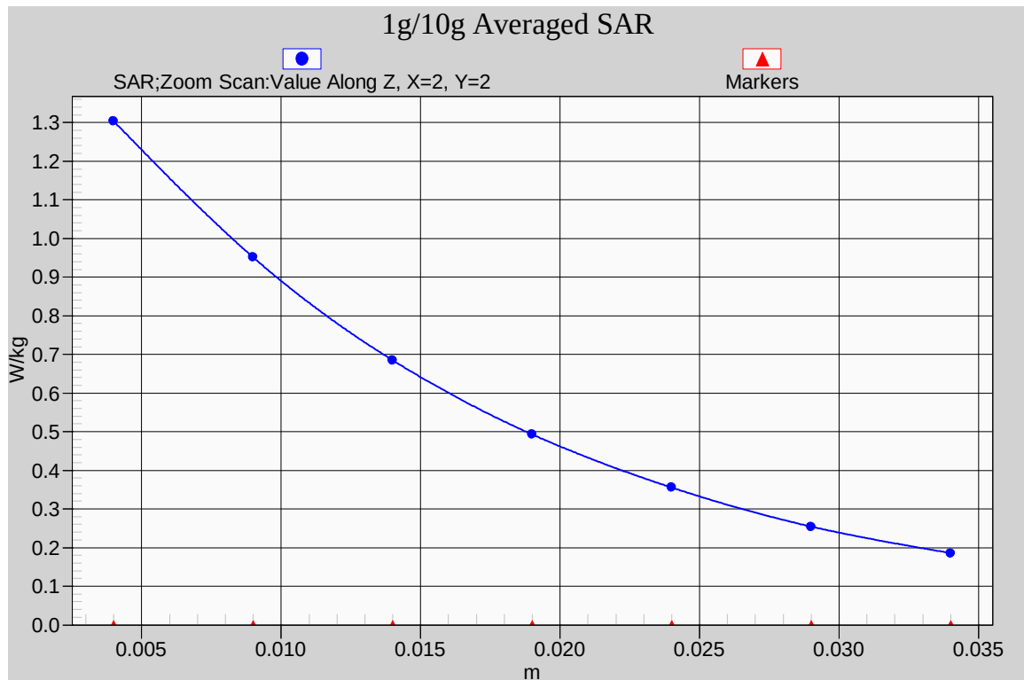
Fig. 11-1 Z-Scan at power reference point (850MHz CH190)
