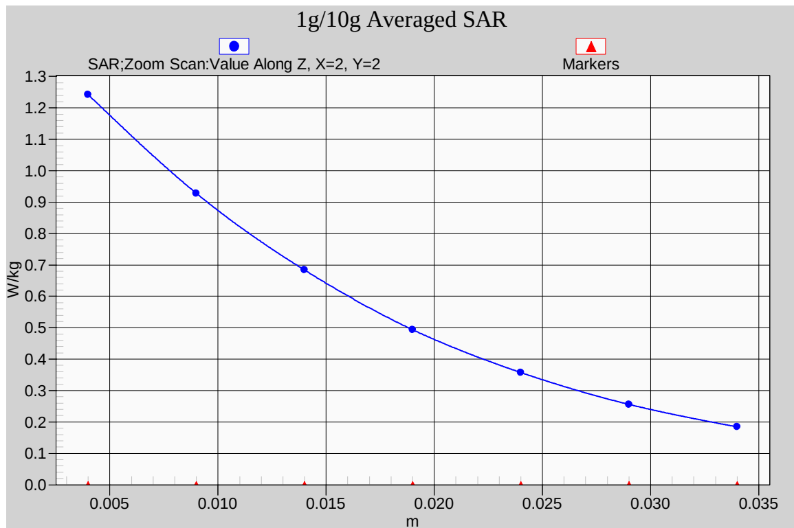
Fig. 3-1 Z-Scan at power reference point (850MHz CH190)
