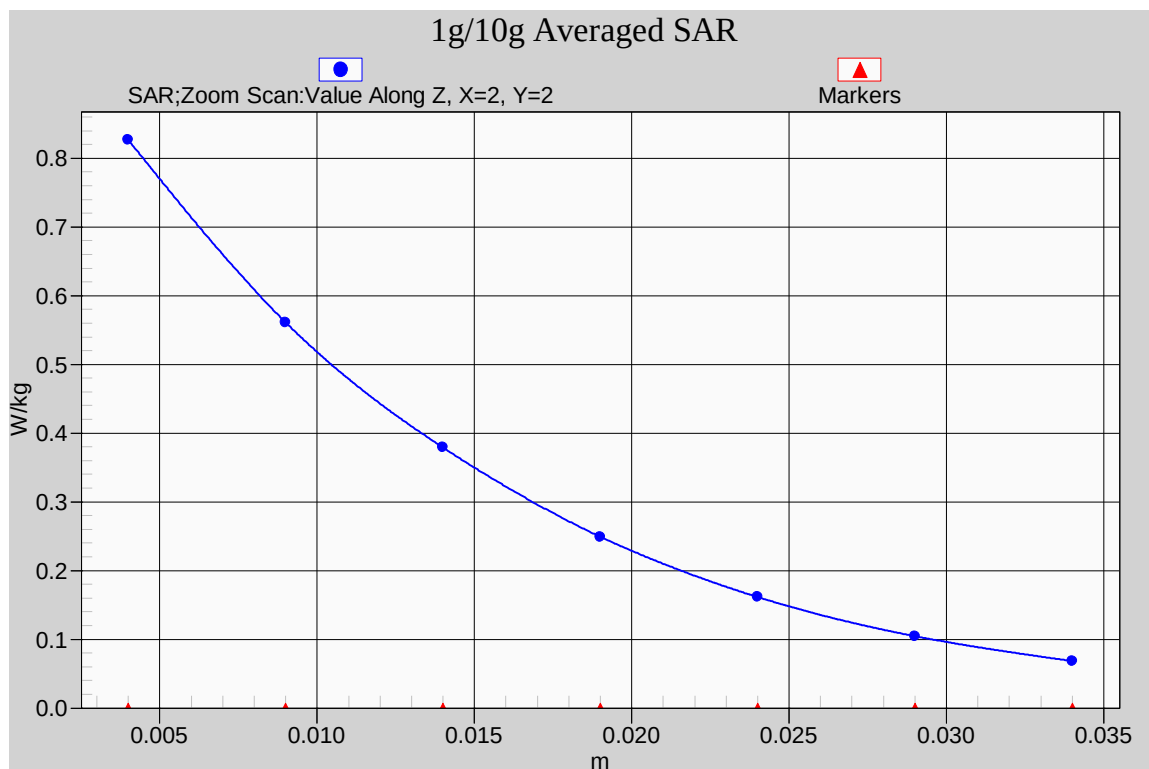
Fig. 27-1 Z-Scan at power reference point (1900 MHz CH512)
