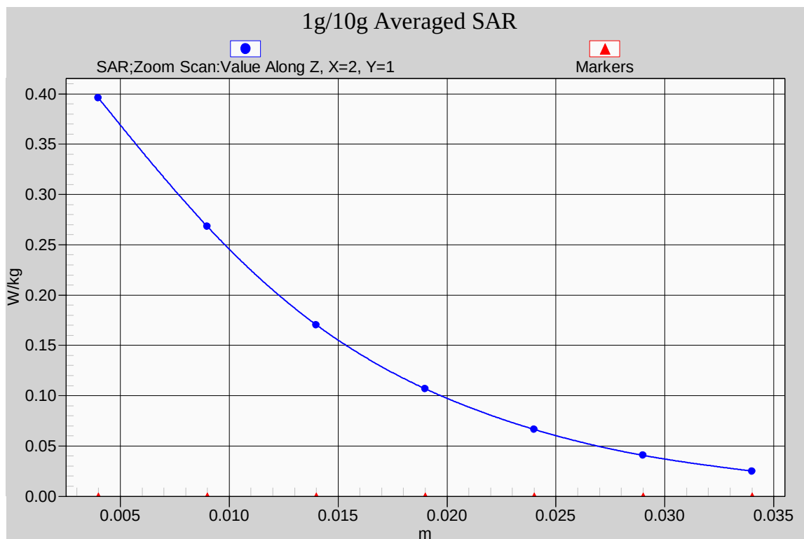
Fig. 22-1 Z-Scan at power reference point (1900MHz CH810)
