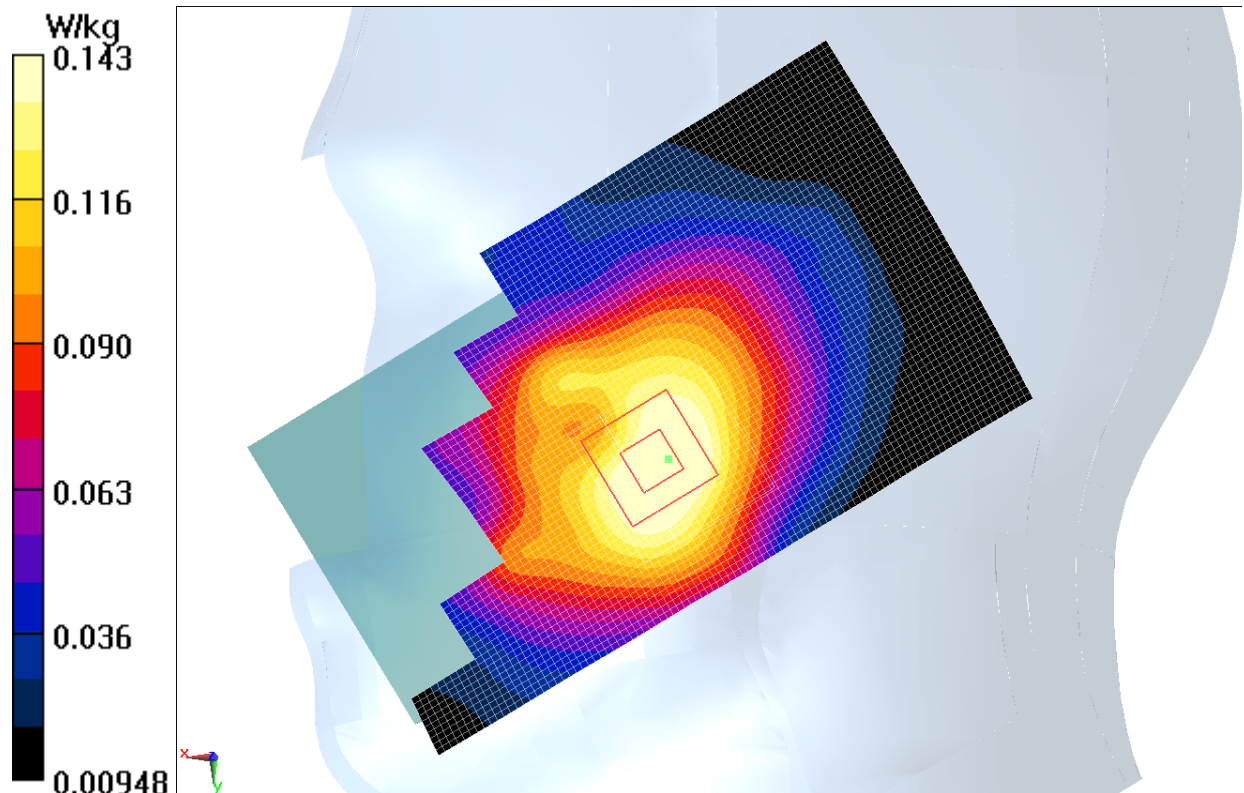
Fig.1 1900 MHz CH190
