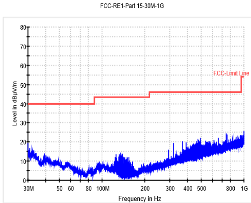
Fig. 170 Radiated Spurious Emission (802.11n-20M, Ch1, 30MHz-1 GHz)
