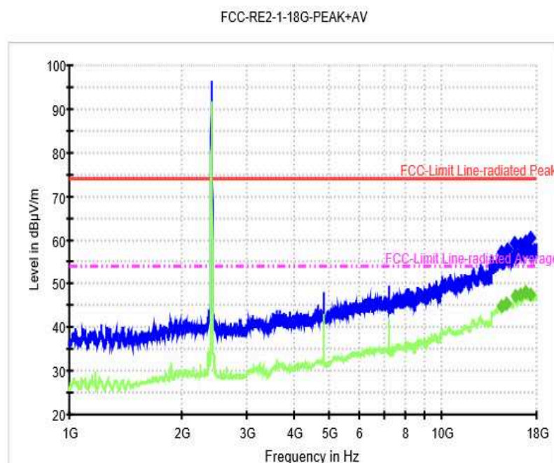
Fig. 155 Radiated Spurious Emission (802.11b, Ch1, 1 GHz-18 GHz)
