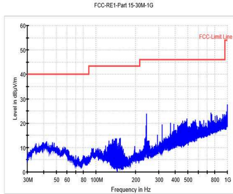
Fig. 156 Radiated Spurious Emission (802.11b, Ch6, 30MHz-1 GHz)
