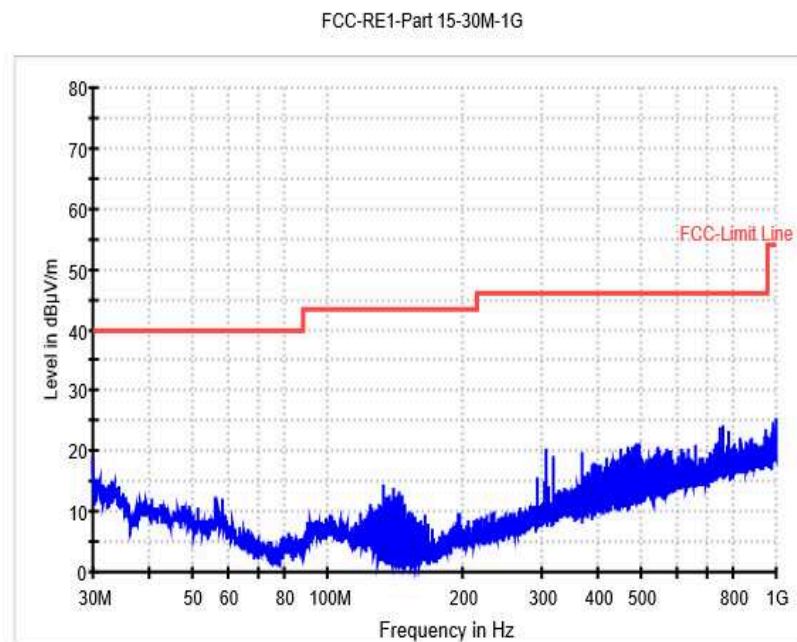
Fig. 182 Radiated Spurious Emission (802.11n-40M, Ch9, 30MHz-1 GHz)
