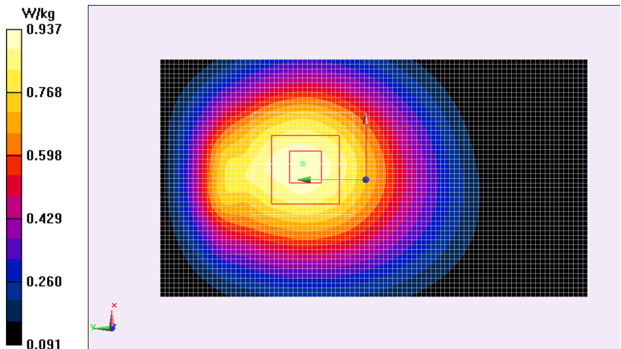
Fig.2 850 MHz CH128
