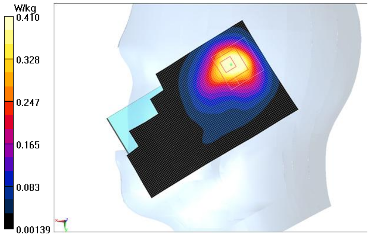
Fig.11 2450 MHz CH11
