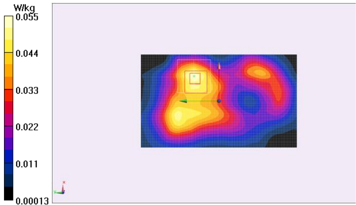
Fig.12 2450 MHz CH11
