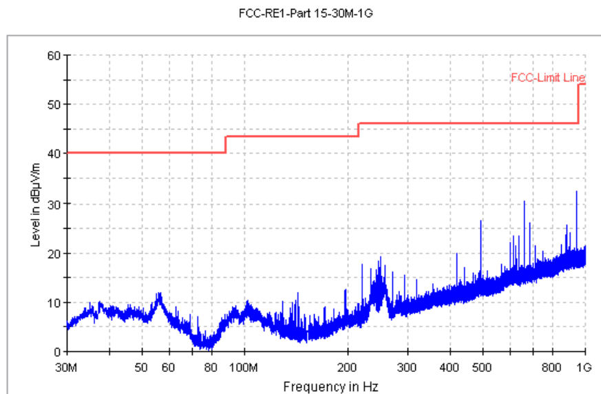
Fig. 66 Radiated Spurious Emission (8DPSK, Ch0, 30 MHz ~1 GHz)
