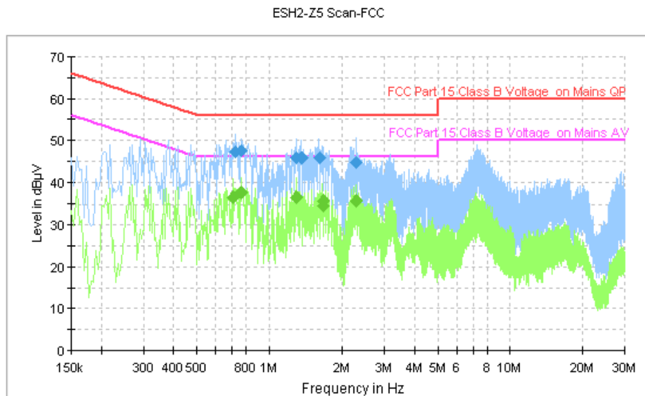
Fig. 99 AC Power line Conducted Emission (Traffic, AE2)
