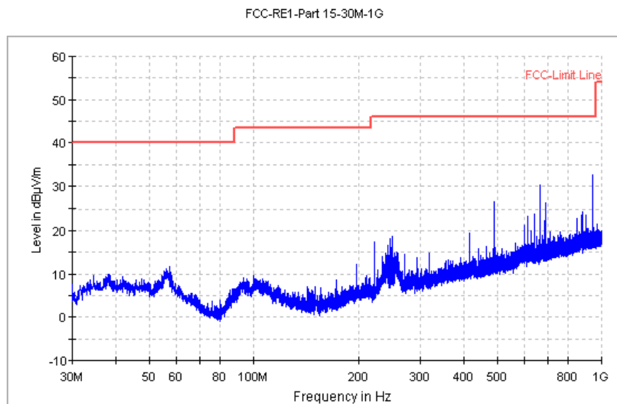
Fig. 70 Radiated Spurious Emission (8DPSK, Ch78, 30 MHz ~1 GHz)
