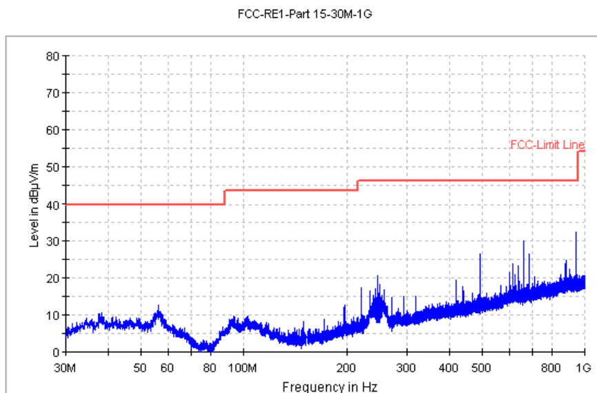
Fig. 50 Radiated Spurious Emission (GFSK, Ch0, 30 MHz ~1 GHz)
