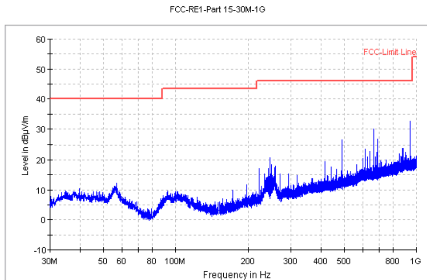
Fig. 68 Radiated Spurious Emission (8DPSK, Ch39, 30 MHz ~1 GHz)
