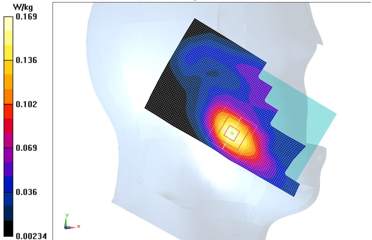
Fig.1 1900 MHz CH661
